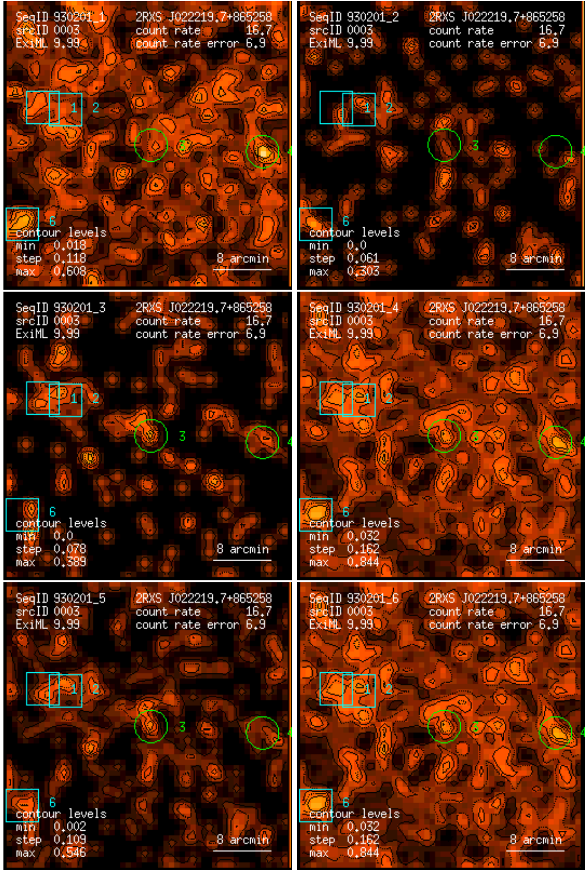
Figure 3: RASS 930201: detection 0003: band rate images, Gaussian filter: (1) PSPC channels 11 – 41, (2) 52 – 90, (3) 91 – 201, (4) 11 – 235, (5) 52 – 201, (6) 11 – 201. Broad band rates in counts/ks. Band rate contour levels in counts/ks/arcmin 2 .
