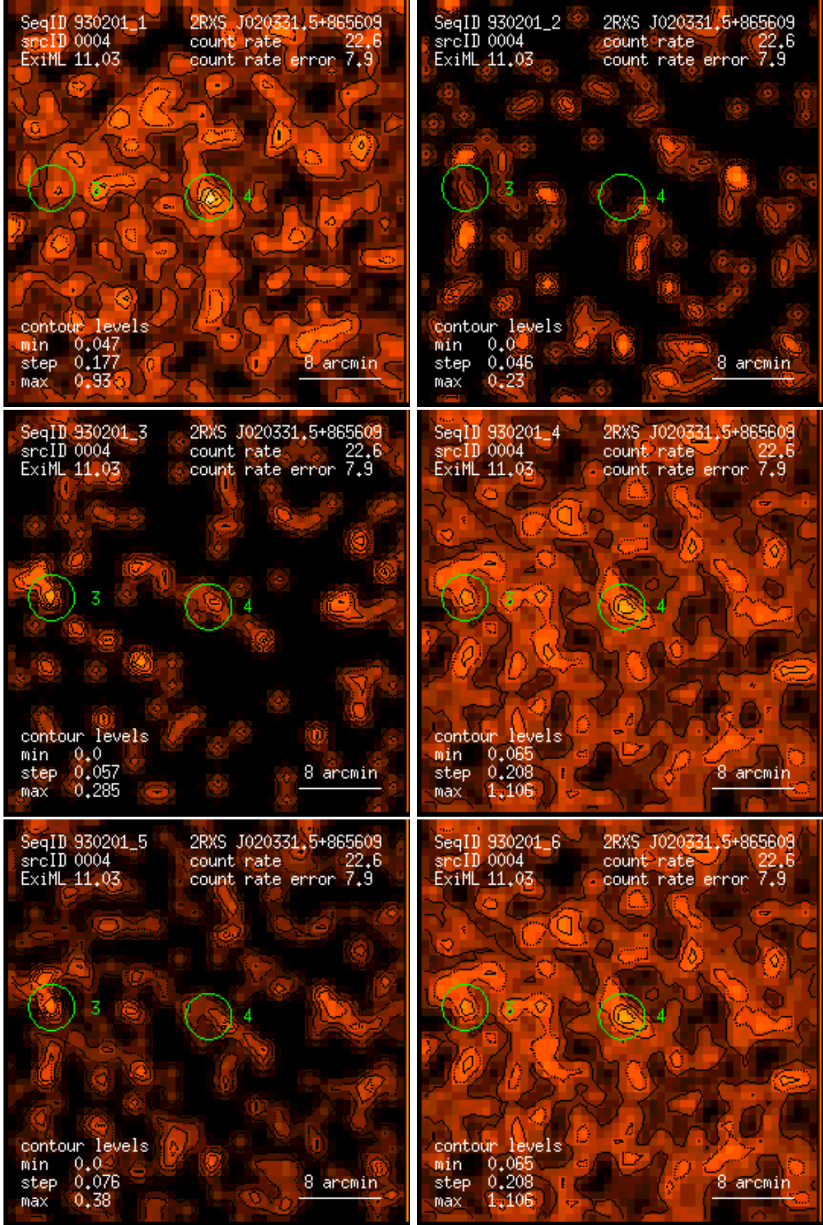
Figure 4: RASS 930201: detection 0004: band rate images, Gaussian filter: (1) PSPC channels 11 – 41, (2) 52 – 90, (3) 91 – 201, (4) 11 – 235, (5) 52 – 201, (6) 11 – 201. Broad band rates in counts/ks. Band rate contour levels in counts/ks/arcmin 2 .
