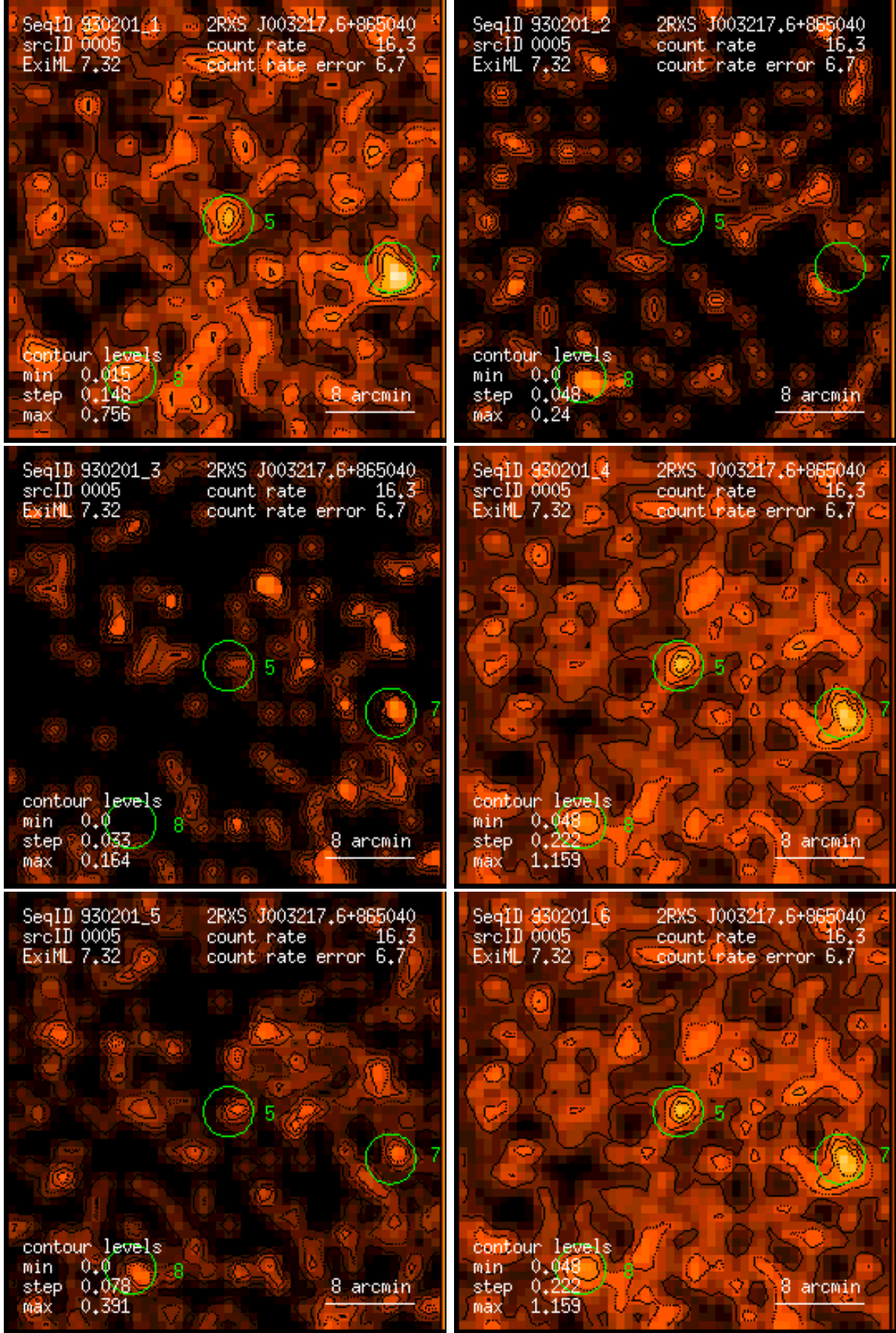
Figure 5: RASS 930201: detection 0005: band rate images, Gaussian filter: (1) PSPC channels 11 – 41, (2) 52 – 90, (3) 91 – 201, (4) 11 – 235, (5) 52 – 201, (6) 11 – 201. Broad band rates in counts/ks. Band rate contour levels in counts/ks/arcmin 2 .
