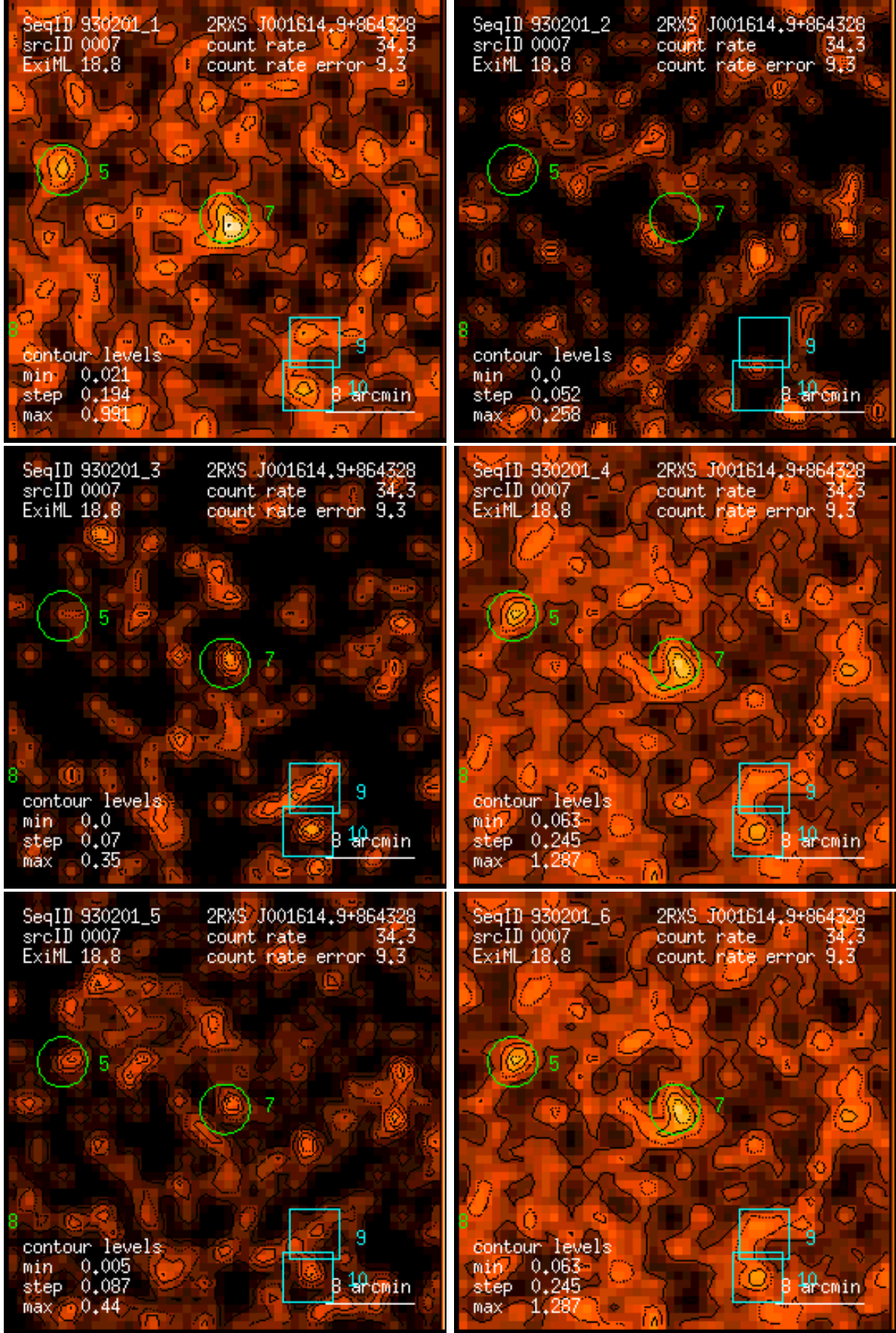
Figure 7: RASS 930201: detection 0007: band rate images, Gaussian filter: (1) PSPC channels 11 – 41, (2) 52 – 90, (3) 91 – 201, (4) 11 – 235, (5) 52 – 201, (6) 11 – 201. Broad band rates in counts/ks. Band rate contour levels in counts/ks/arcmin 2 .
