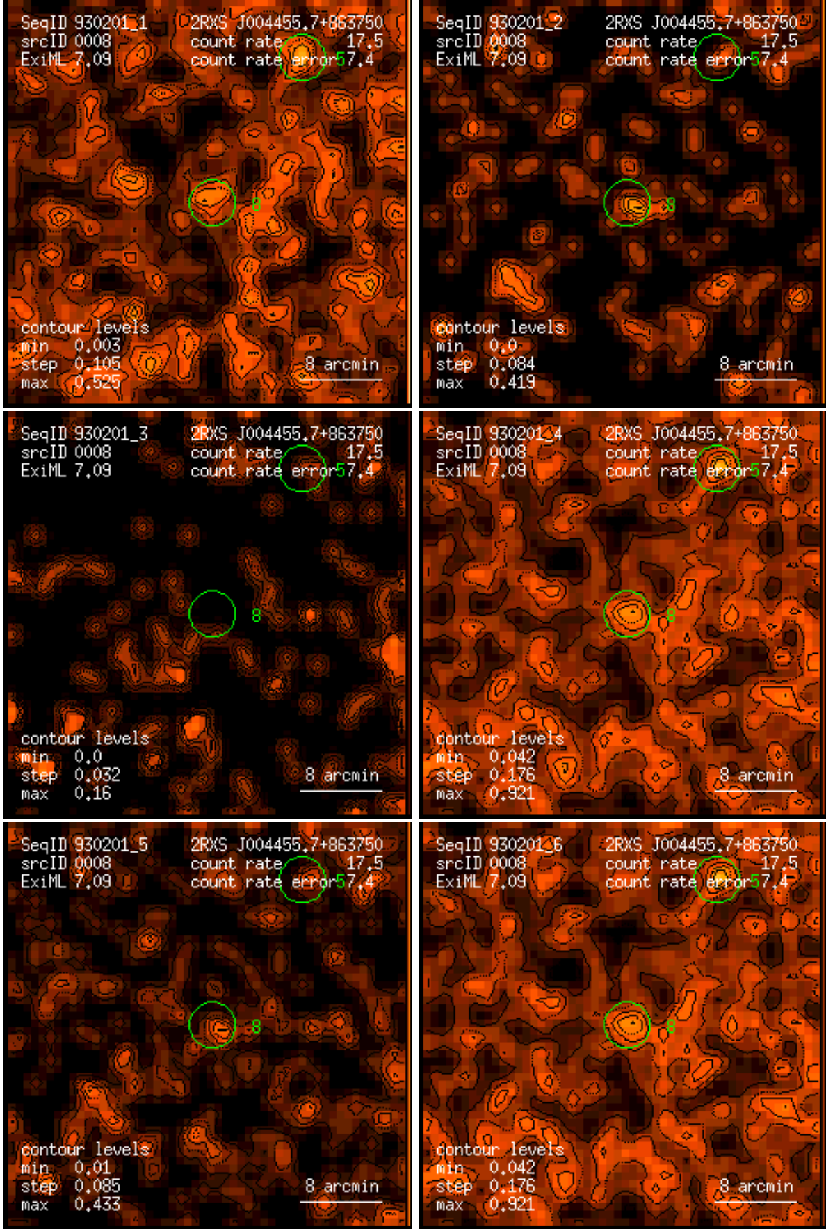
Figure 8: RASS 930201: detection 0008: band rate images, Gaussian filter: (1) PSPC channels 11 – 41, (2) 52 – 90, (3) 91 – 201, (4) 11 – 235, (5) 52 – 201, (6) 11 – 201. Broad band rates in counts/ks. Band rate contour levels in counts/ks/arcmin 2 .
