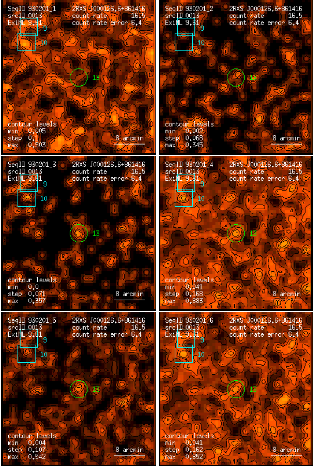
Figure 13: RASS 930201: detection 0013: band rate images, Gaussian filter: (1) PSPC channels 11 – 41, (2) 52 – 90, (3) 91 – 201, (4) 11 – 235, (5) 52 – 201, (6) 11 – 201. Broad band rates in counts/ks. Band rate contour levels in counts/ks/arcmin 2 .
