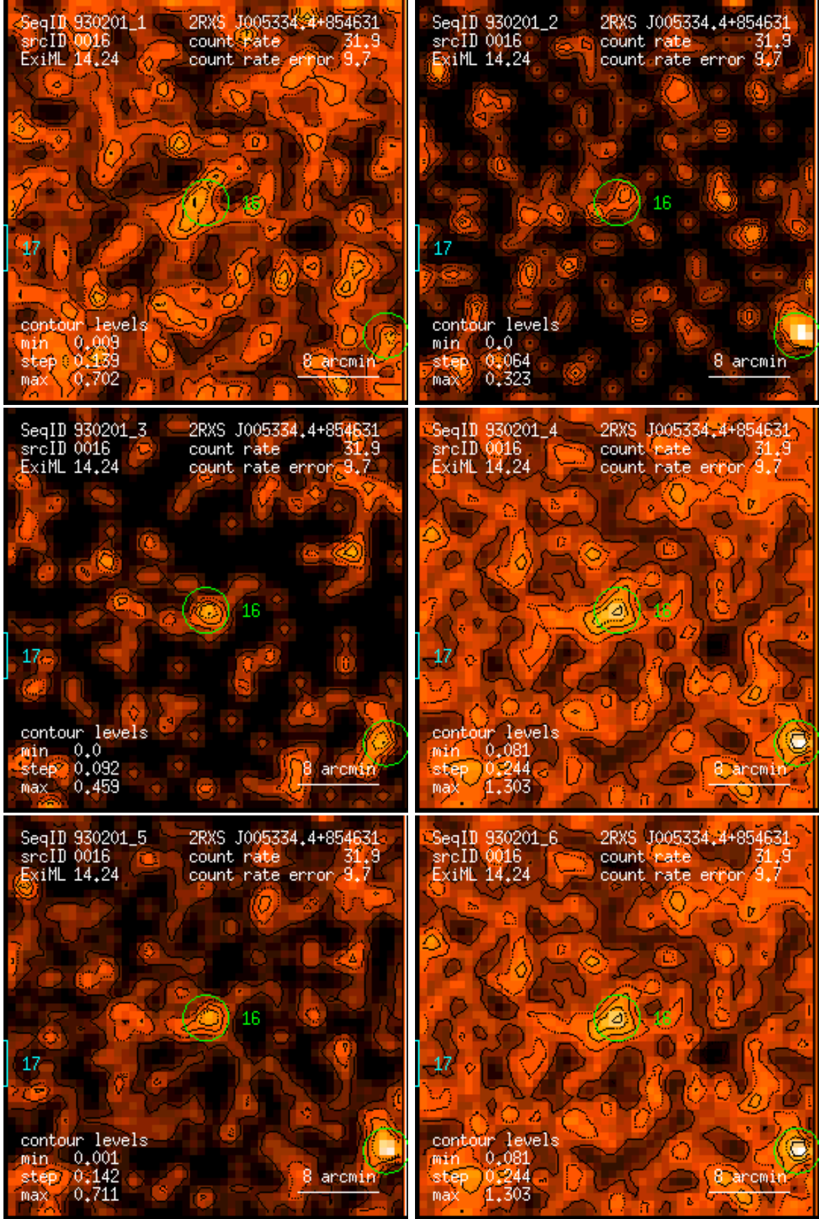
Figure 16: RASS 930201: detection 0016: band rate images, Gaussian filter: (1) PSPC channels 11 – 41, (2) 52 – 90, (3) 91 – 201, (4) 11 – 235, (5) 52 – 201, (6) 11 – 201. Broad band rates in counts/ks. Band rate contour levels in counts/ks/arcmin 2 .
