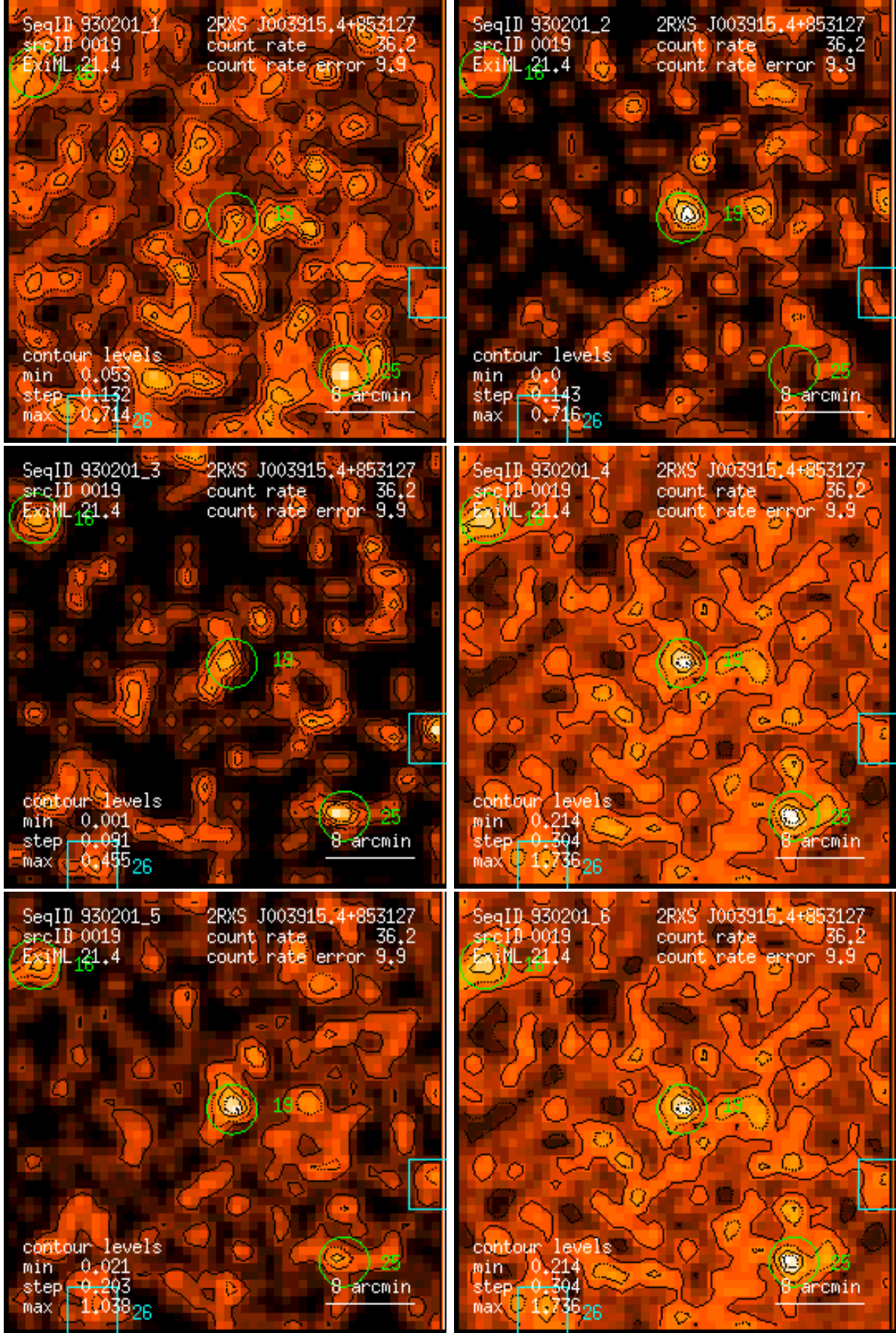
Figure 19: RASS 930201: detection 0019: band rate images, Gaussian filter: (1) PSPC channels 11 – 41, (2) 52 – 90, (3) 91 – 201, (4) 11 – 235, (5) 52 – 201, (6) 11 – 201. Broad band rates in counts/ks. Band rate contour levels in counts/ks/arcmin 2 .
