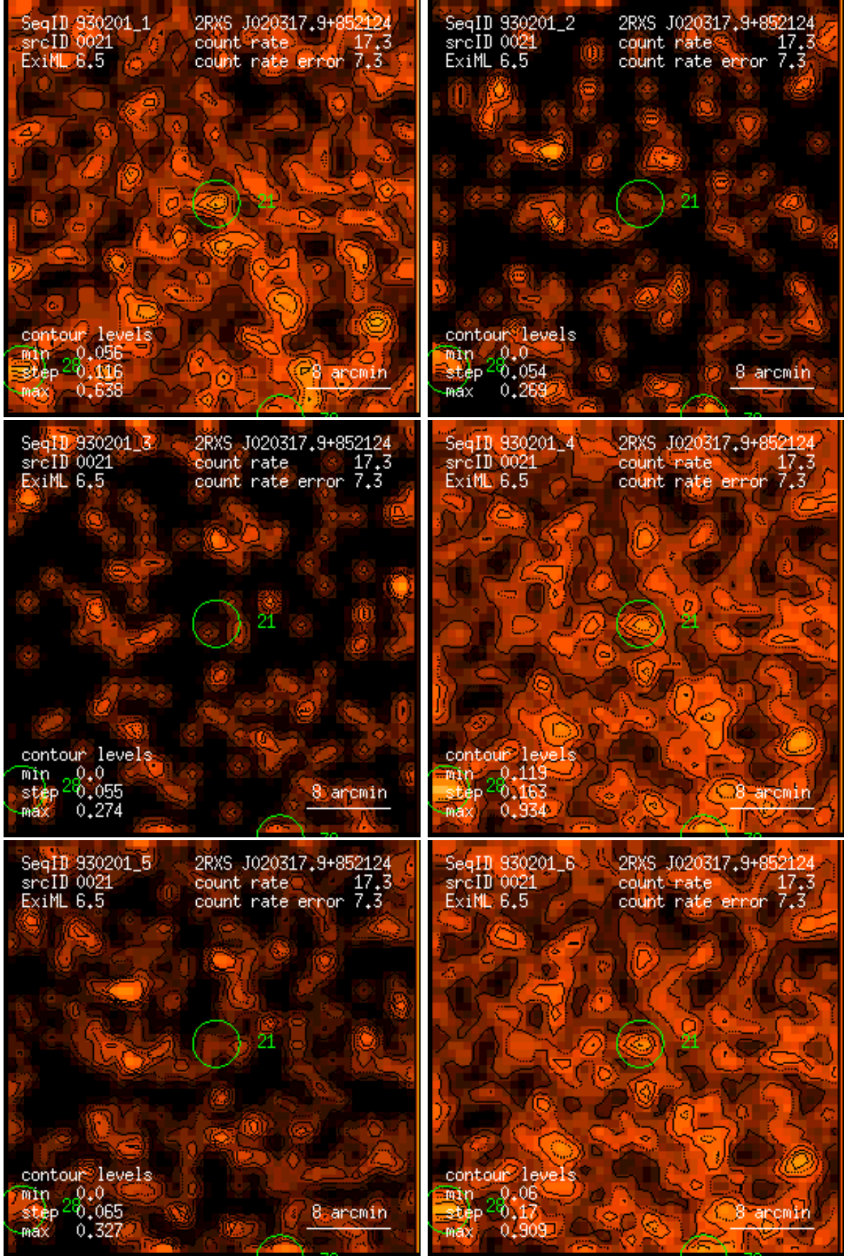
Figure 21: RASS 930201: detection 0021: band rate images, Gaussian filter: (1) PSPC channels 11 – 41, (2) 52 – 90, (3) 91 – 201, (4) 11 – 235, (5) 52 – 201, (6) 11 – 201. Broad band rates in counts/ks. Band rate contour levels in counts/ks/arcmin 2 .
