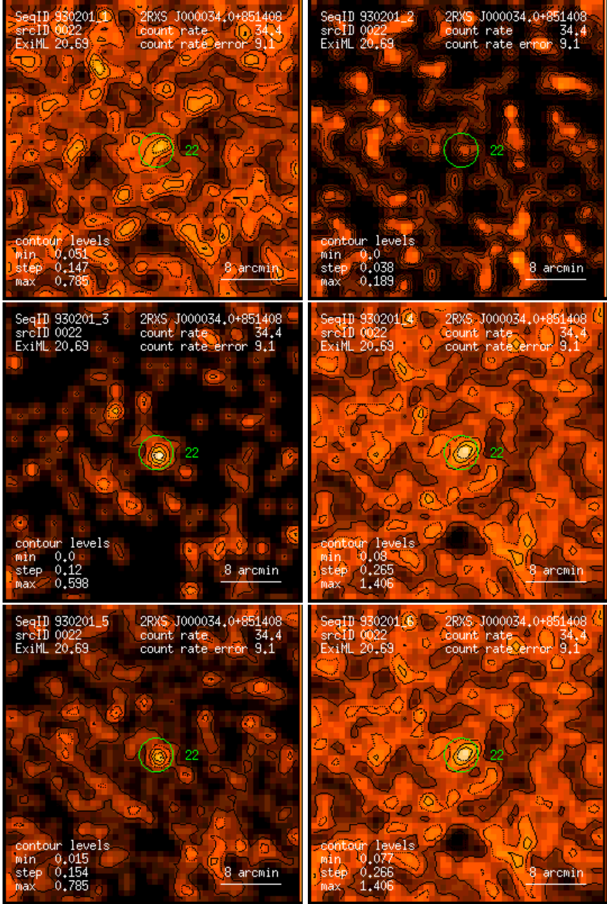
Figure 22: RASS 930201: detection 0022: band rate images, Gaussian filter: (1) PSPC channels 11 – 41, (2) 52 – 90, (3) 91 – 201, (4) 11 – 235, (5) 52 – 201, (6) 11 – 201. Broad band rates in counts/ks. Band rate contour levels in counts/ks/arcmin 2 .
