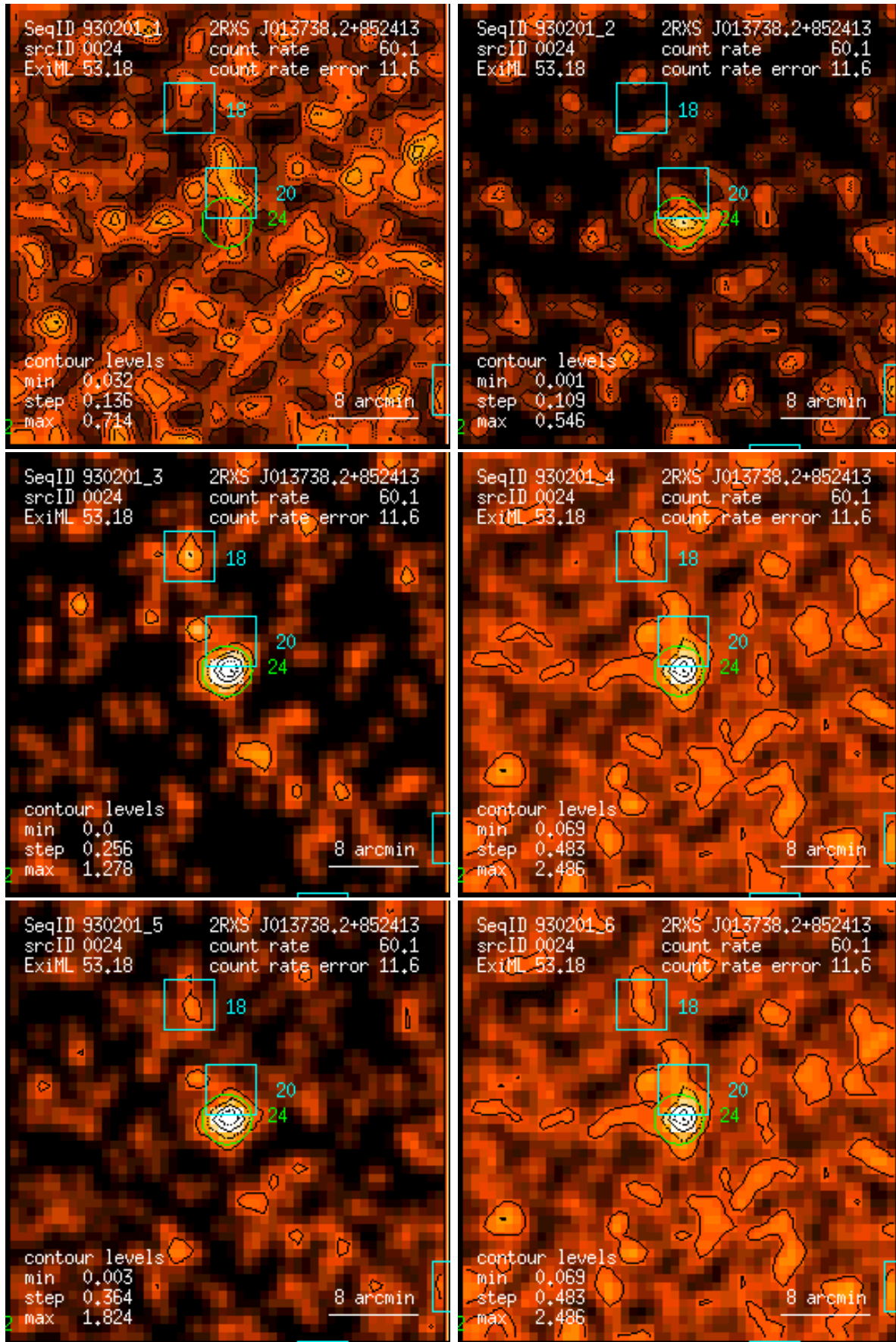
Figure 24: RASS 930201: detection 0024: band rate images, Gaussian filter: (1) PSPC channels 11 – 41, (2) 52 – 90, (3) 91 – 201, (4) 11 – 235, (5) 52 – 201, (6) 11 – 201. Broad band rates in counts/ks. Band rate contour levels in counts/ks/arcmin 2 .
