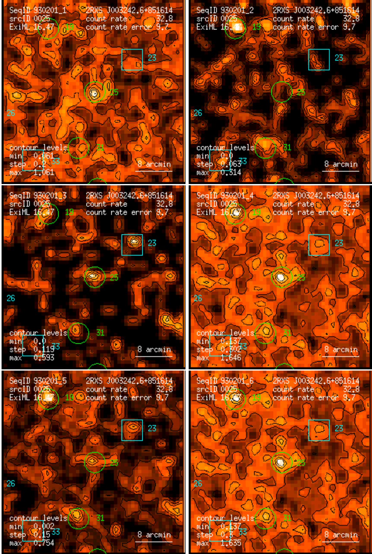
Figure 25: RASS 930201: detection 0025: band rate images, Gaussian filter: (1) PSPC channels 11 – 41, (2) 52 – 90, (3) 91 – 201, (4) 11 – 235, (5) 52 – 201, (6) 11 – 201. Broad band rates in counts/ks. Band rate contour levels in counts/ks/arcmin 2 .
