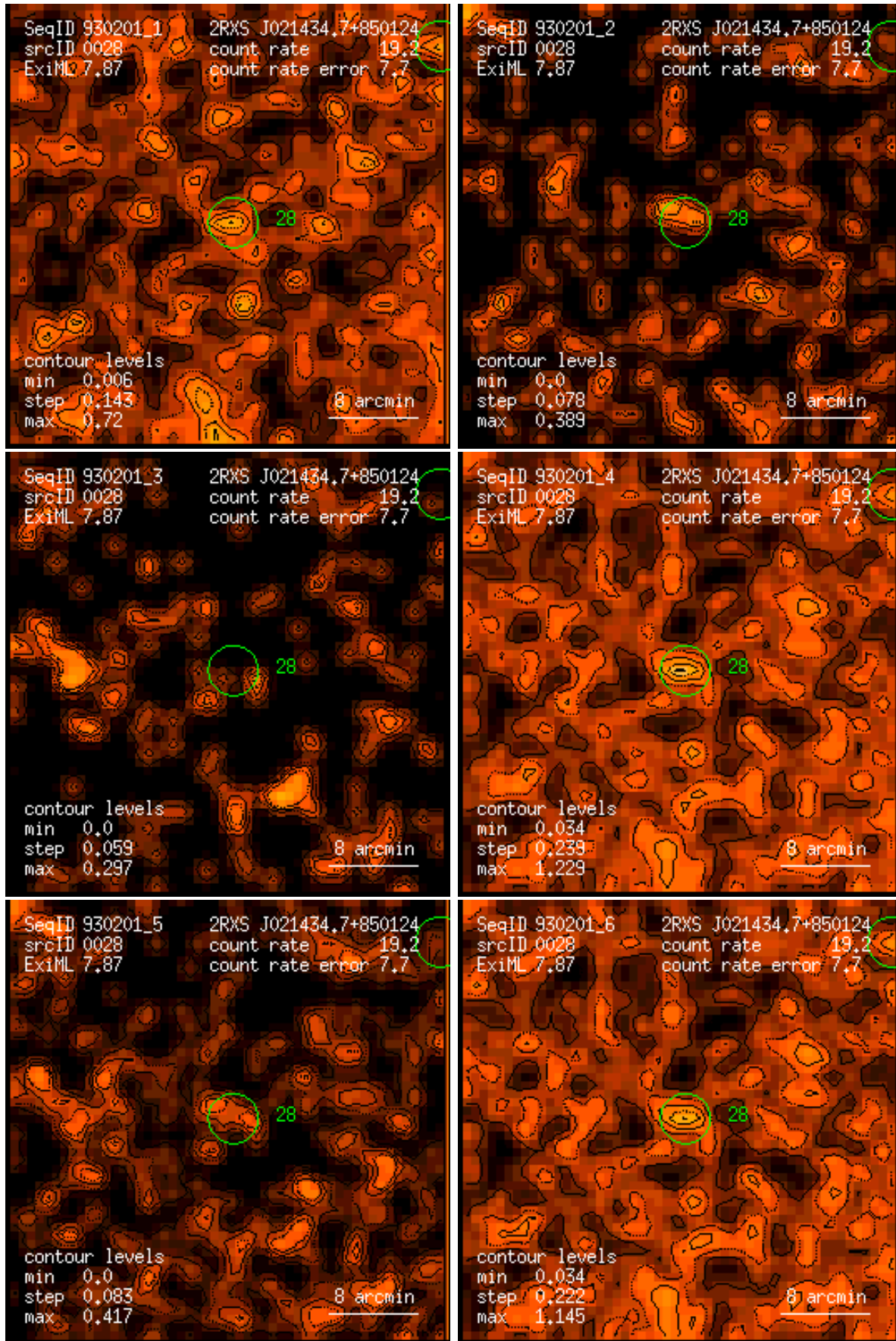
Figure 28: RASS 930201: detection 0028: band rate images, Gaussian filter: (1) PSPC channels 11 – 41, (2) 52 – 90, (3) 91 – 201, (4) 11 – 235, (5) 52 – 201, (6) 11 – 201. Broad band rates in counts/ks. Band rate contour levels in counts/ks/arcmin 2 .
