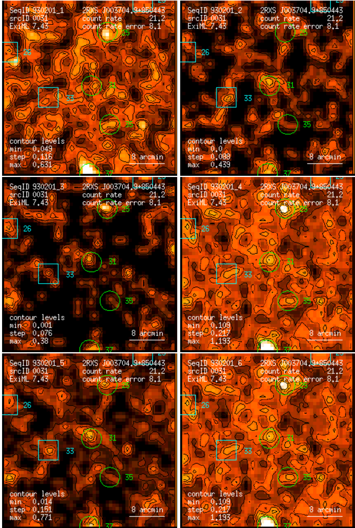
Figure 31: RASS 930201: detection 0031: band rate images, Gaussian filter: (1) PSPC channels 11 – 41, (2) 52 – 90, (3) 91 – 201, (4) 11 – 235, (5) 52 – 201, (6) 11 – 201. Broad band rates in counts/ks. Band rate contour levels in counts/ks/arcmin 2 .
