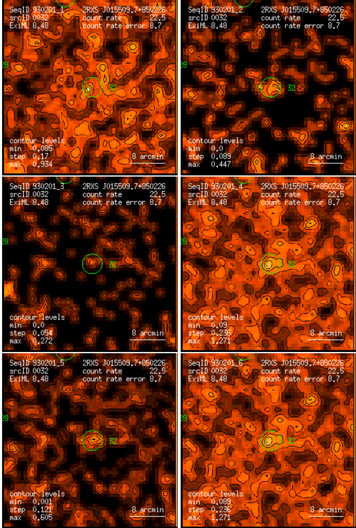
Figure 32: RASS 930201: detection 0032: band rate images, Gaussian filter: (1) PSPC channels 11 – 41, (2) 52 – 90, (3) 91 – 201, (4) 11 – 235, (5) 52 – 201, (6) 11 – 201. Broad band rates in counts/ks. Band rate contour levels in counts/ks/arcmin 2 .
