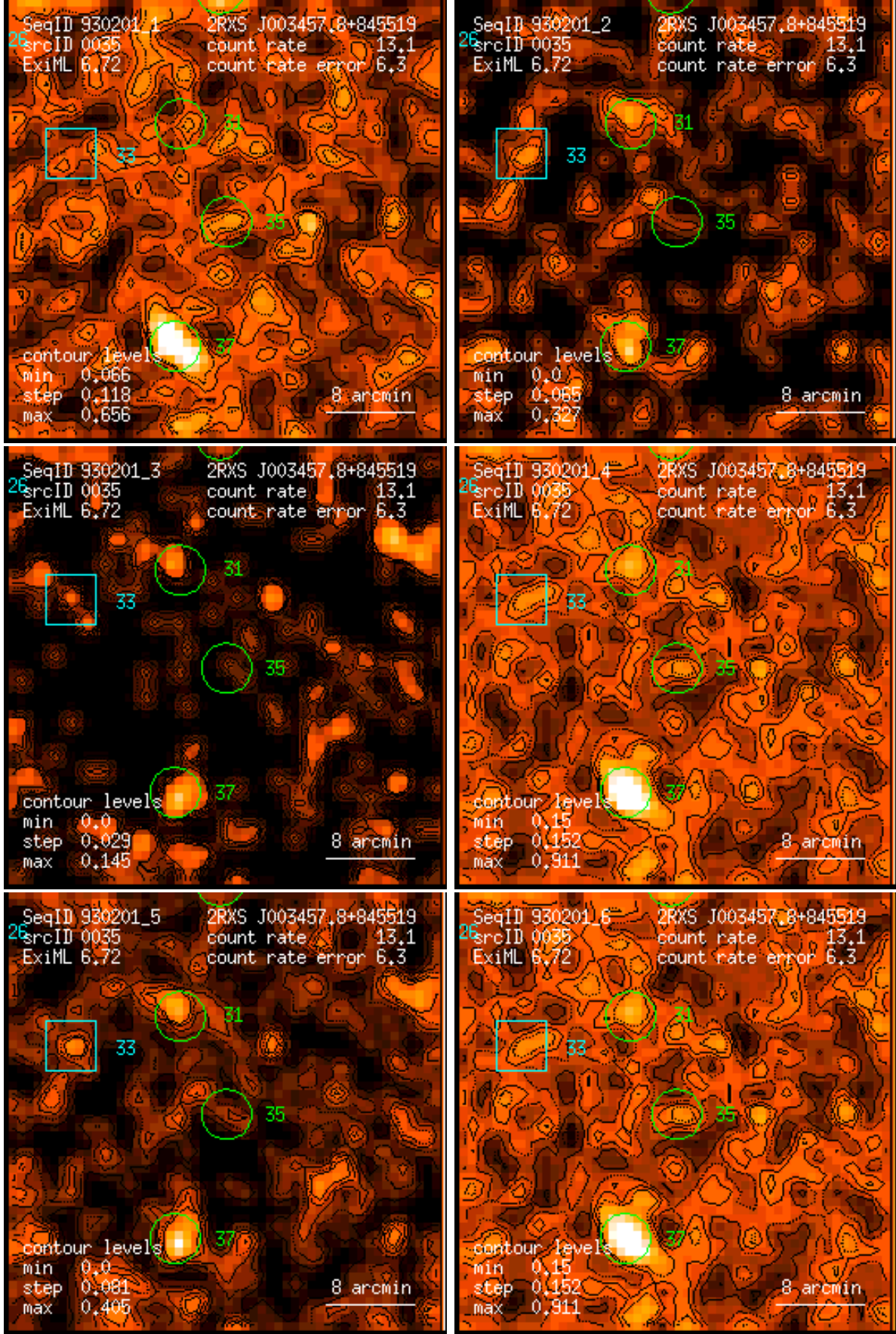
Figure 35: RASS 930201: detection 0035: band rate images, Gaussian filter: (1) PSPC channels 11 – 41, (2) 52 – 90, (3) 91 – 201, (4) 11 – 235, (5) 52 – 201, (6) 11 – 201. Broad band rates in counts/ks. Band rate contour levels in counts/ks/arcmin 2 .
