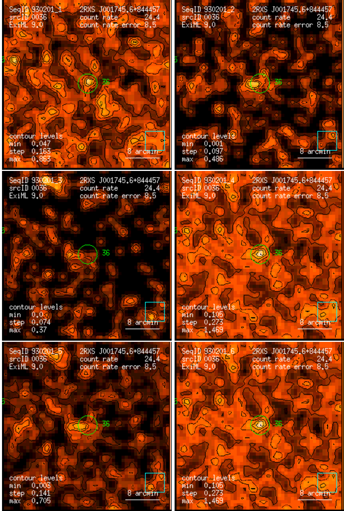
Figure 36: RASS 930201: detection 0036: band rate images, Gaussian filter: (1) PSPC channels 11 – 41, (2) 52 – 90, (3) 91 – 201, (4) 11 – 235, (5) 52 – 201, (6) 11 – 201. Broad band rates in counts/ks. Band rate contour levels in counts/ks/arcmin 2 .
