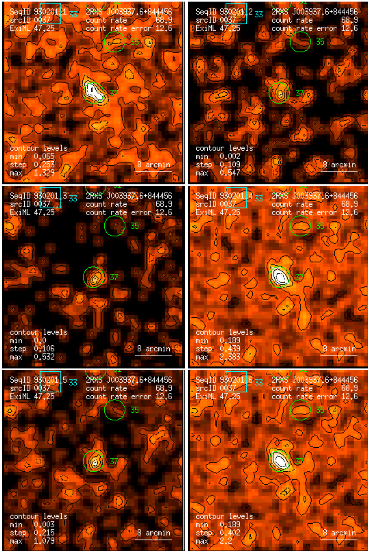
Figure 37: RASS 930201: detection 0037: band rate images, Gaussian filter: (1) PSPC channels 11 – 41, (2) 52 – 90, (3) 91 – 201, (4) 11 – 235, (5) 52 – 201, (6) 11 – 201. Broad band rates in counts/ks. Band rate contour levels in counts/ks/arcmin 2 .
