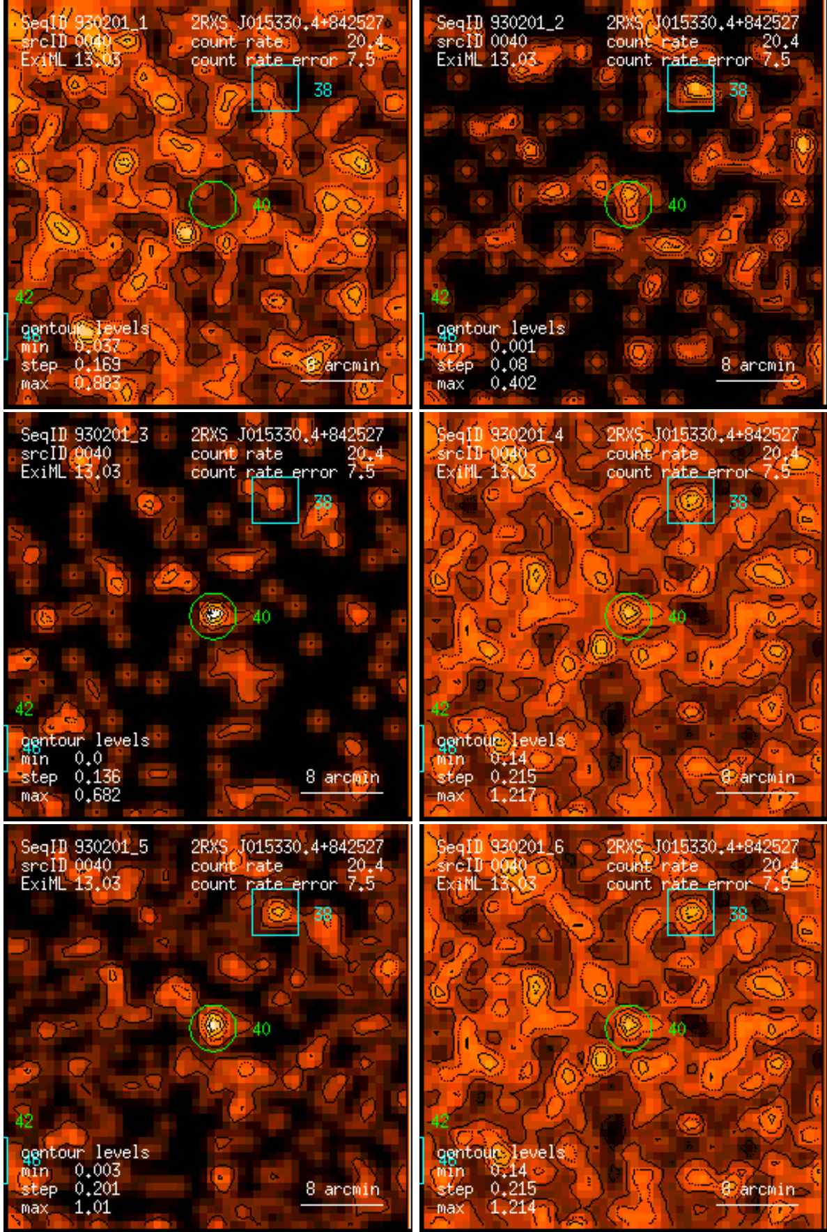
Figure 40: RASS 930201: detection 0040: band rate images, Gaussian filter: (1) PSPC channels 11 – 41, (2) 52 – 90, (3) 91 – 201, (4) 11 – 235, (5) 52 – 201, (6) 11 – 201. Broad band rates in counts/ks. Band rate contour levels in counts/ks/arcmin 2 .
