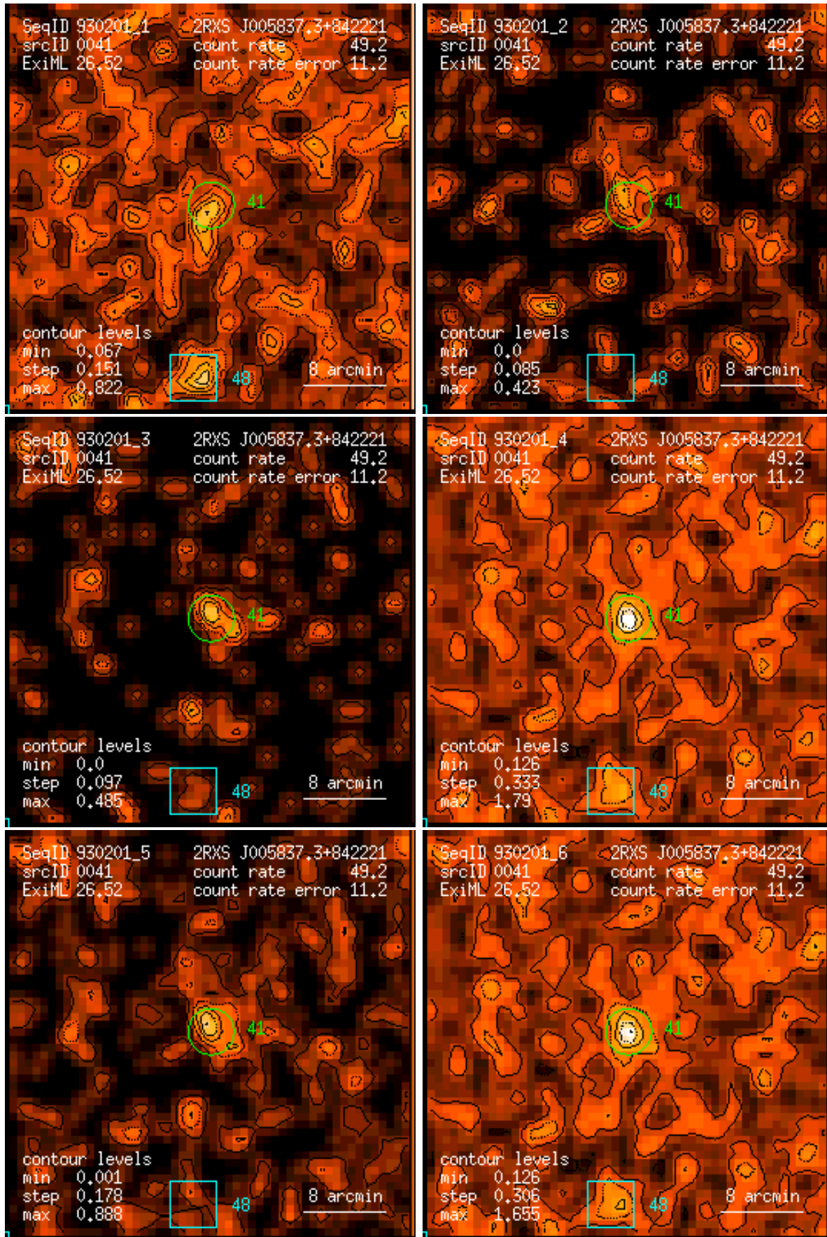
Figure 41: RASS 930201: detection 0041: band rate images, Gaussian filter: (1) PSPC channels 11 – 41, (2) 52 – 90, (3) 91 – 201, (4) 11 – 235, (5) 52 – 201, (6) 11 – 201. Broad band rates in counts/ks. Band rate contour levels in counts/ks/arcmin 2 .
