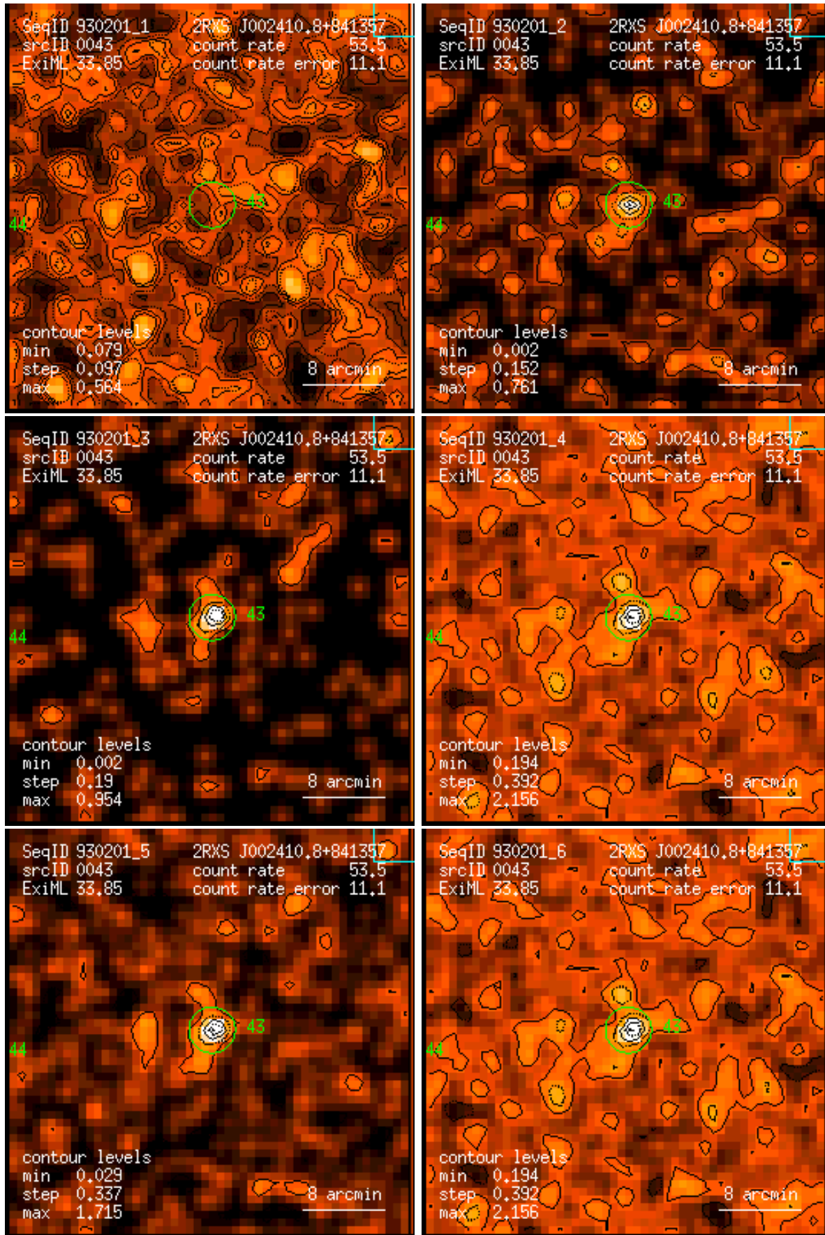
Figure 43: RASS 930201: detection 0043: band rate images, Gaussian filter: (1) PSPC channels 11 – 41, (2) 52 – 90, (3) 91 – 201, (4) 11 – 235, (5) 52 – 201, (6) 11 – 201. Broad band rates in counts/ks. Band rate contour levels in counts/ks/arcmin 2 .
