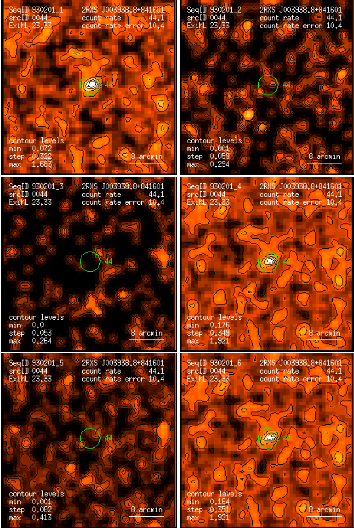
Figure 44: RASS 930201: detection 0044: band rate images, Gaussian filter: (1) PSPC channels 11 – 41, (2) 52 – 90, (3) 91 – 201, (4) 11 – 235, (5) 52 – 201, (6) 11 – 201. Broad band rates in counts/ks. Band rate contour levels in counts/ks/arcmin 2 .
