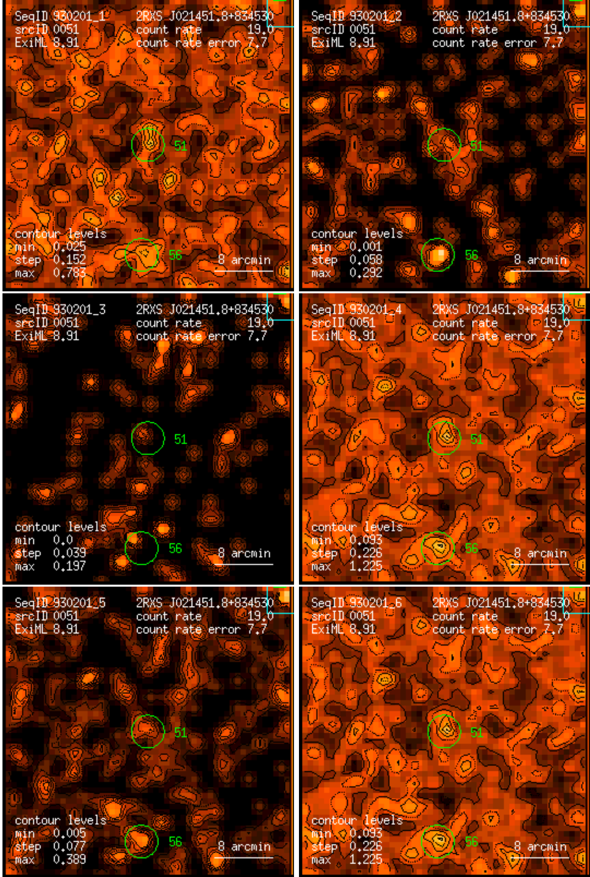
Figure 51: RASS 930201: detection 0051: band rate images, Gaussian filter: (1) PSPC channels 11 – 41, (2) 52 – 90, (3) 91 – 201, (4) 11 – 235, (5) 52 – 201, (6) 11 – 201. Broad band rates in counts/ks. Band rate contour levels in counts/ks/arcmin 2 .
