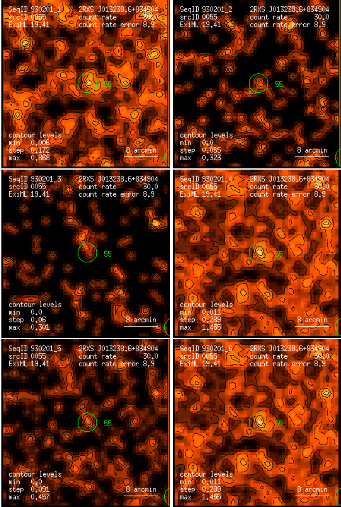
Figure 55: RASS 930201: detection 0055: band rate images, Gaussian filter: (1) PSPC channels 11 – 41, (2) 52 – 90, (3) 91 – 201, (4) 11 – 235, (5) 52 – 201, (6) 11 – 201. Broad band rates in counts/ks. Band rate contour levels in counts/ks/arcmin 2 .
