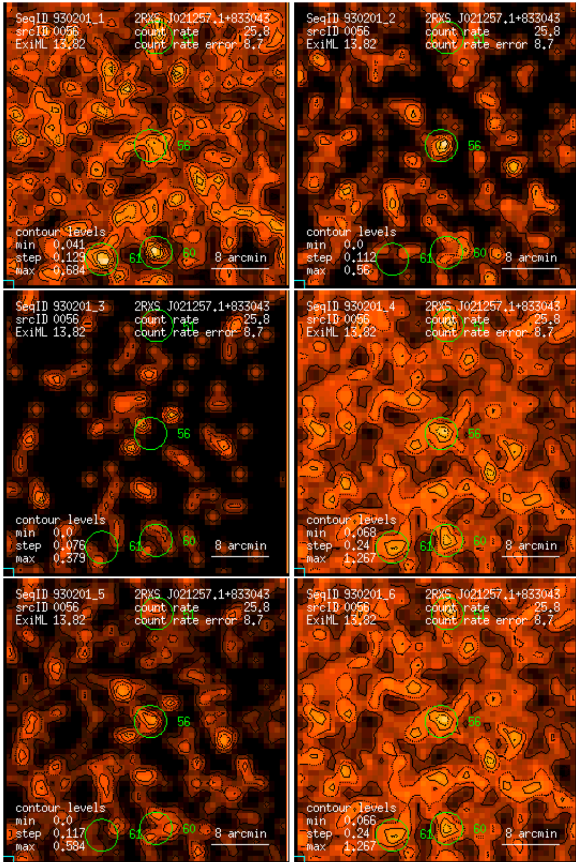
Figure 56: RASS 930201: detection 0056: band rate images, Gaussian filter: (1) PSPC channels 11 – 41, (2) 52 – 90, (3) 91 – 201, (4) 11 – 235, (5) 52 – 201, (6) 11 – 201. Broad band rates in counts/ks. Band rate contour levels in counts/ks/arcmin 2 .
