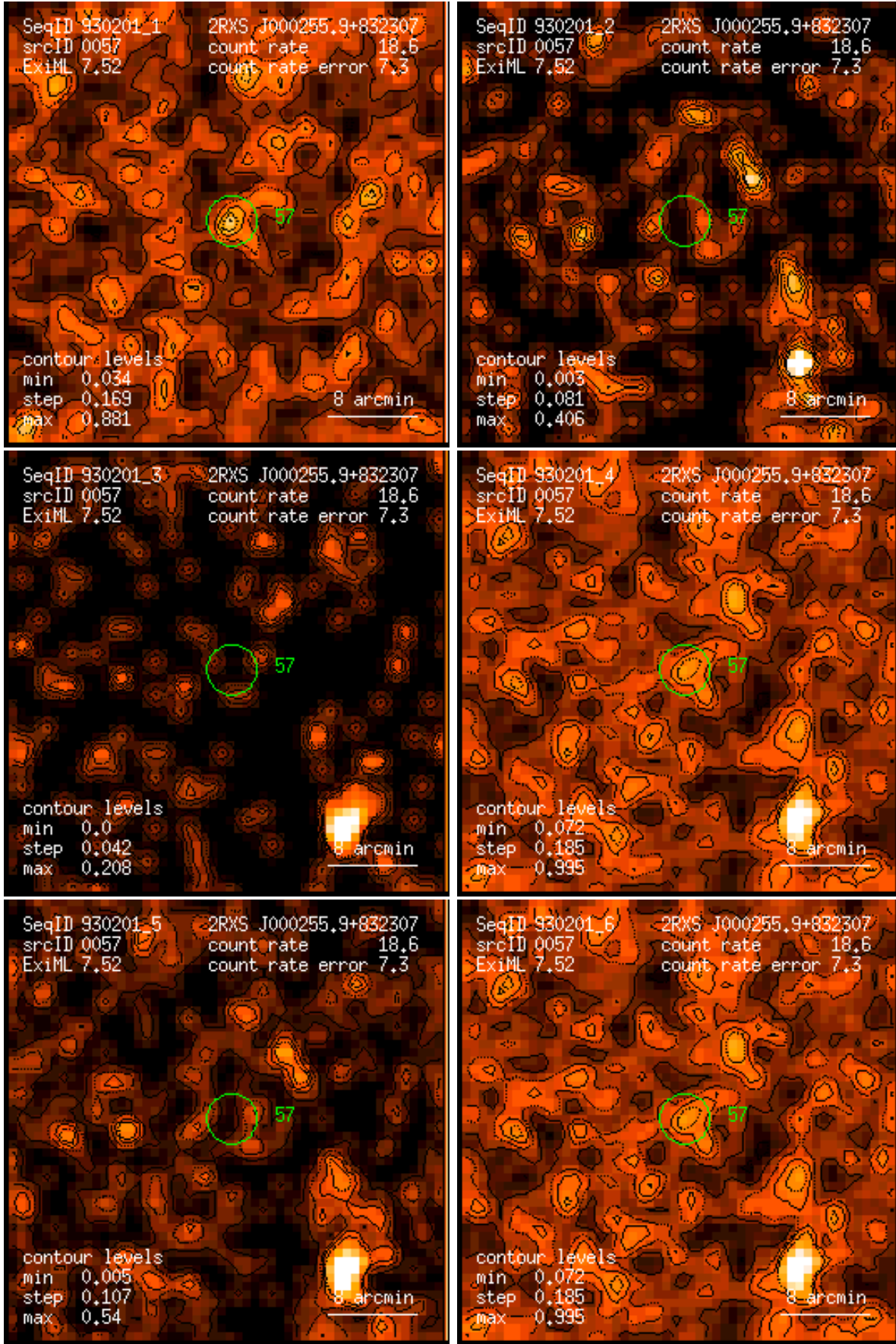
Figure 57: RASS 930201: detection 0057: band rate images, Gaussian filter: (1) PSPC channels 11 – 41, (2) 52 – 90, (3) 91 – 201, (4) 11 – 235, (5) 52 – 201, (6) 11 – 201. Broad band rates in counts/ks. Band rate contour levels in counts/ks/arcmin 2 .
