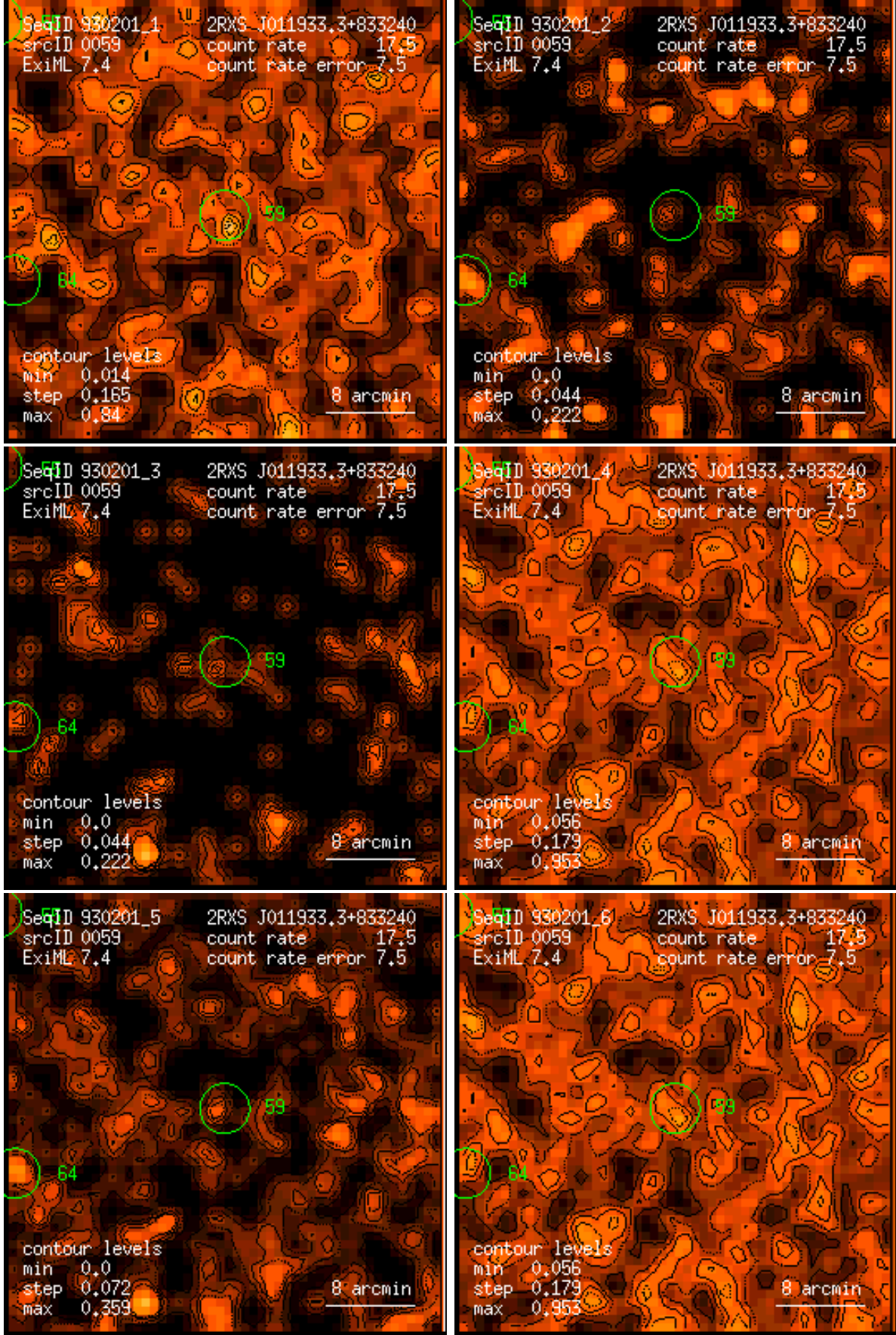
Figure 59: RASS 930201: detection 0059: band rate images, Gaussian filter: (1) PSPC channels 11 – 41, (2) 52 – 90, (3) 91 – 201, (4) 11 – 235, (5) 52 – 201, (6) 11 – 201. Broad band rates in counts/ks. Band rate contour levels in counts/ks/arcmin 2 .
