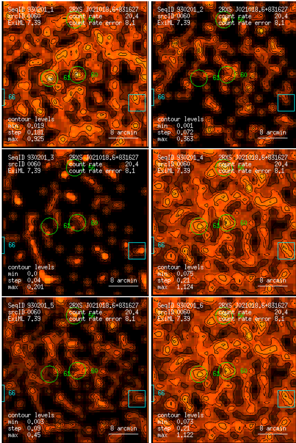
Figure 60: RASS 930201: detection 0060: band rate images, Gaussian filter: (1) PSPC channels 11 – 41, (2) 52 – 90, (3) 91 – 201, (4) 11 – 235, (5) 52 – 201, (6) 11 – 201. Broad band rates in counts/ks. Band rate contour levels in counts/ks/arcmin 2 .
