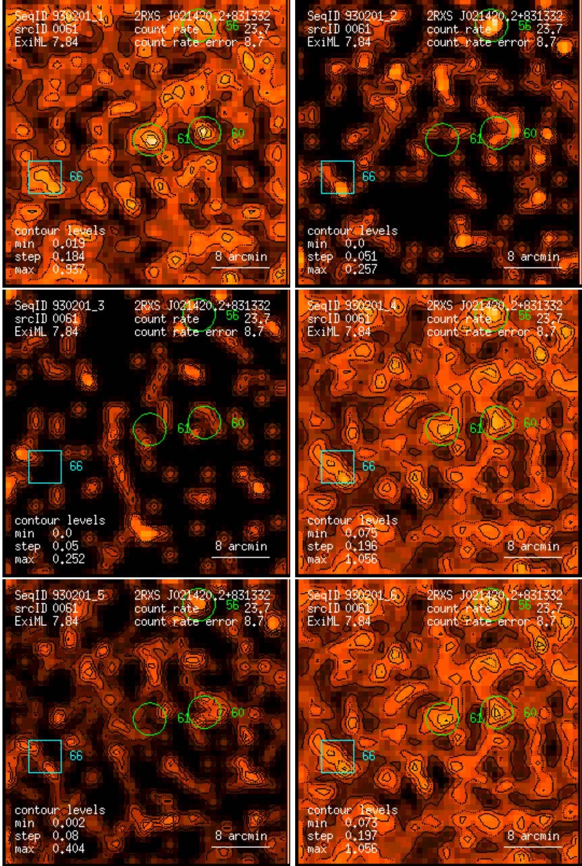
Figure 61: RASS 930201: detection 0061: band rate images, Gaussian filter: (1) PSPC channels 11 – 41, (2) 52 – 90, (3) 91 – 201, (4) 11 – 235, (5) 52 – 201, (6) 11 – 201. Broad band rates in counts/ks. Band rate contour levels in counts/ks/arcmin 2 .
