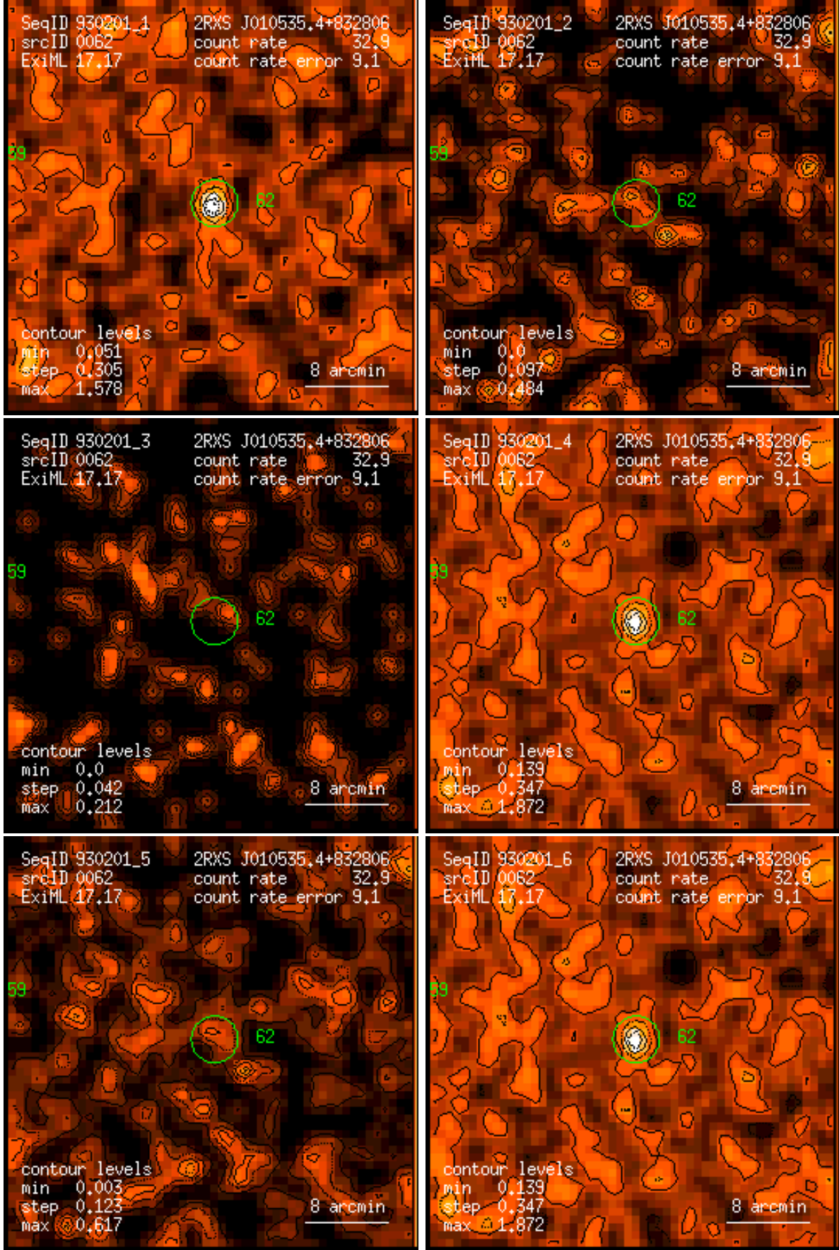
Figure 62: RASS 930201: detection 0062: band rate images, Gaussian filter: (1) PSPC channels 11 – 41, (2) 52 – 90, (3) 91 – 201, (4) 11 – 235, (5) 52 – 201, (6) 11 – 201. Broad band rates in counts/ks. Band rate contour levels in counts/ks/arcmin 2 .
