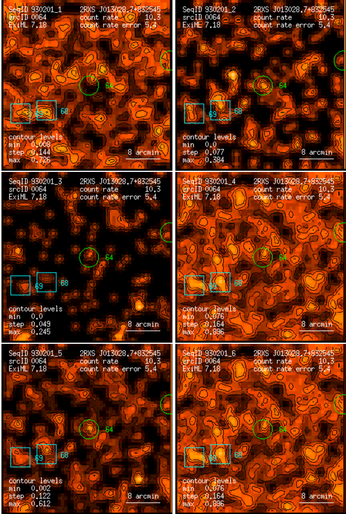
Figure 64: RASS 930201: detection 0064: band rate images, Gaussian filter: (1) PSPC channels 11 – 41, (2) 52 – 90, (3) 91 – 201, (4) 11 – 235, (5) 52 – 201, (6) 11 – 201. Broad band rates in counts/ks. Band rate contour levels in counts/ks/arcmin 2 .
