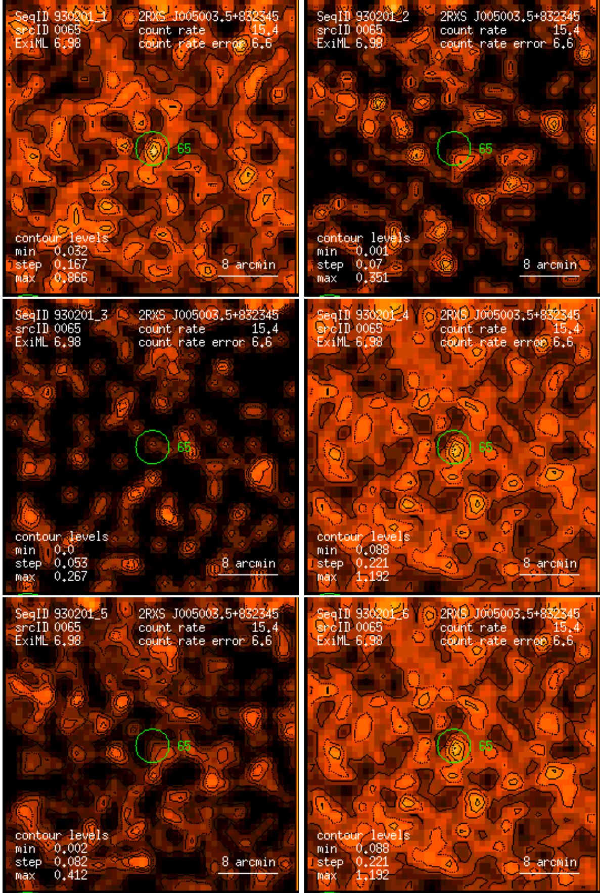
Figure 65: RASS 930201: detection 0065: band rate images, Gaussian filter: (1) PSPC channels 11 – 41, (2) 52 – 90, (3) 91 – 201, (4) 11 – 235, (5) 52 – 201, (6) 11 – 201. Broad band rates in counts/ks. Band rate contour levels in counts/ks/arcmin 2 .
