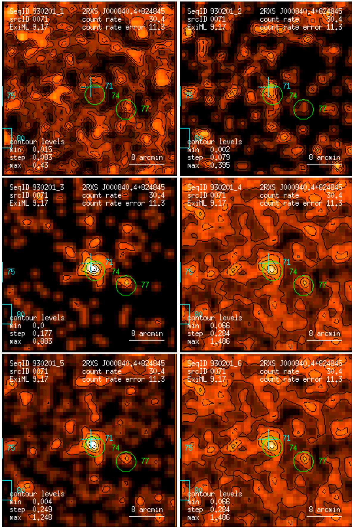
Figure 71: RASS 930201: detection 0071: band rate images, Gaussian filter: (1) PSPC channels 11 – 41, (2) 52 – 90, (3) 91 – 201, (4) 11 – 235, (5) 52 – 201, (6) 11 – 201. Broad band rates in counts/ks. Band rate contour levels in counts/ks/arcmin 2 .
