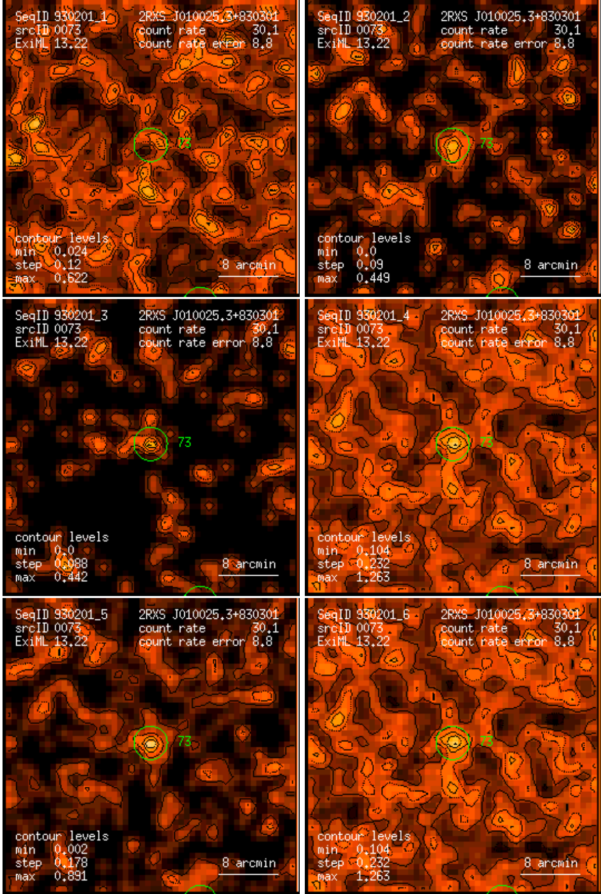
Figure 73: RASS 930201: detection 0073: band rate images, Gaussian filter: (1) PSPC channels 11 – 41, (2) 52 – 90, (3) 91 – 201, (4) 11 – 235, (5) 52 – 201, (6) 11 – 201. Broad band rates in counts/ks. Band rate contour levels in counts/ks/arcmin 2 .
