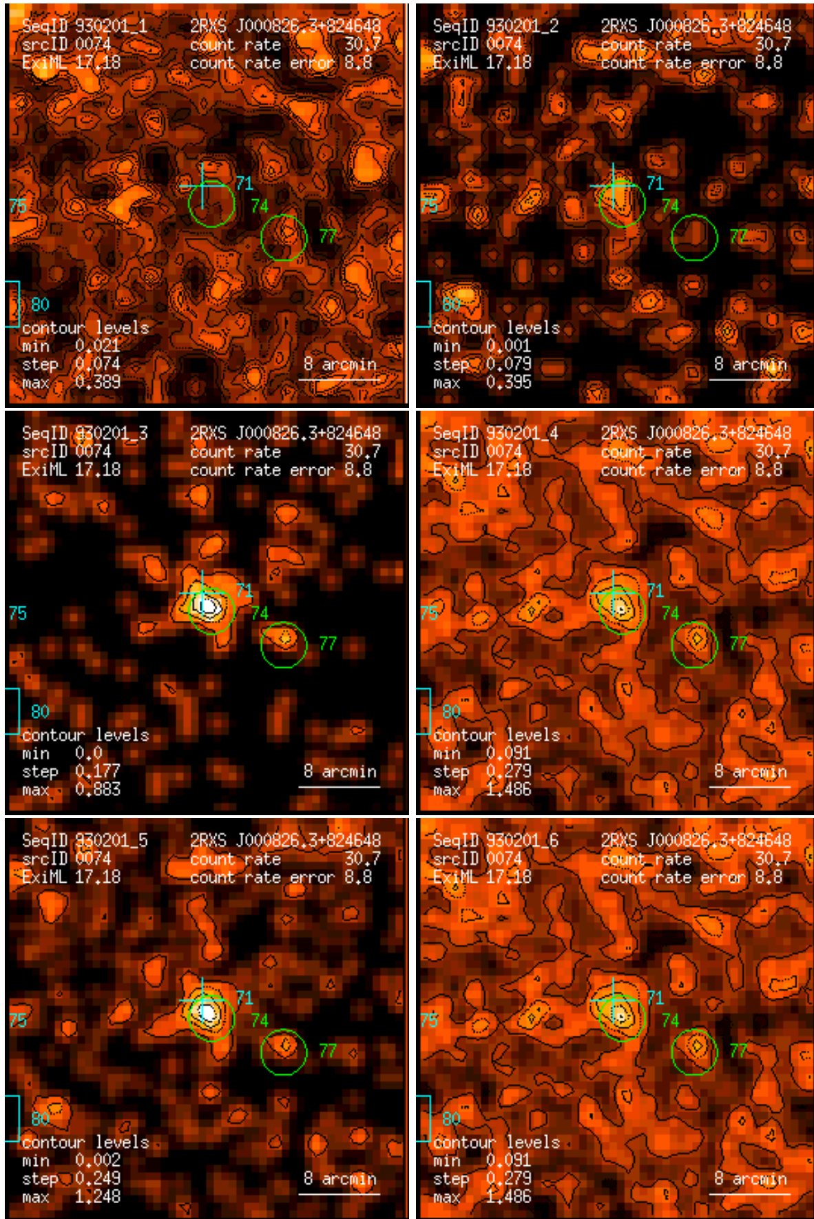
Figure 74: RASS 930201: detection 0074: band rate images, Gaussian filter: (1) PSPC channels 11 – 41, (2) 52 – 90, (3) 91 – 201, (4) 11 – 235, (5) 52 – 201, (6) 11 – 201. Broad band rates in counts/ks. Band rate contour levels in counts/ks/arcmin 2 .
