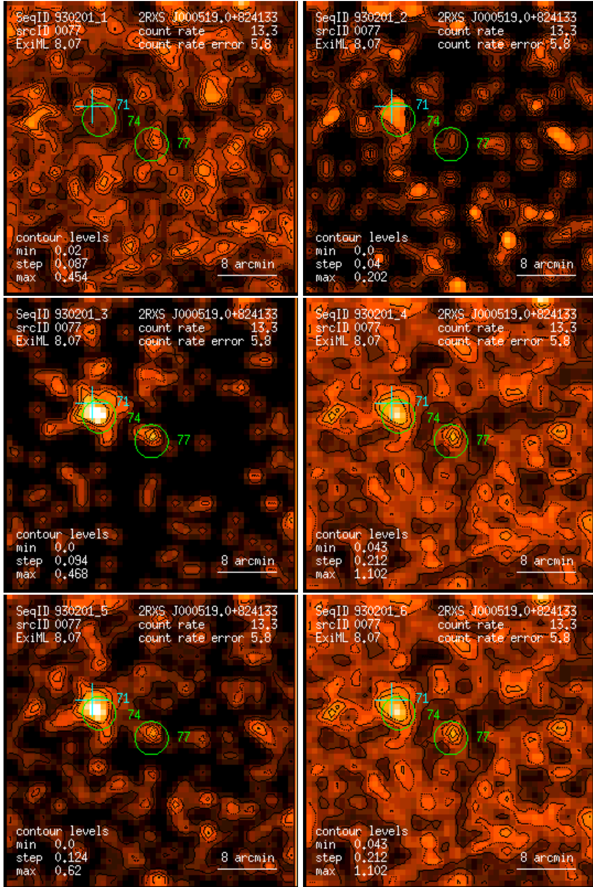
Figure 77: RASS 930201: detection 0077: band rate images, Gaussian filter: (1) PSPC channels 11 – 41, (2) 52 – 90, (3) 91 – 201, (4) 11 – 235, (5) 52 – 201, (6) 11 – 201. Broad band rates in counts/ks. Band rate contour levels in counts/ks/arcmin 2 .
