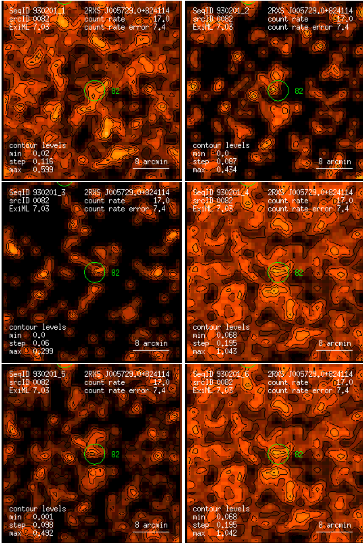
Figure 82: RASS 930201: detection 0082: band rate images, Gaussian filter: (1) PSPC channels 11 – 41, (2) 52 – 90, (3) 91 – 201, (4) 11 – 235, (5) 52 – 201, (6) 11 – 201. Broad band rates in counts/ks. Band rate contour levels in counts/ks/arcmin 2 .
