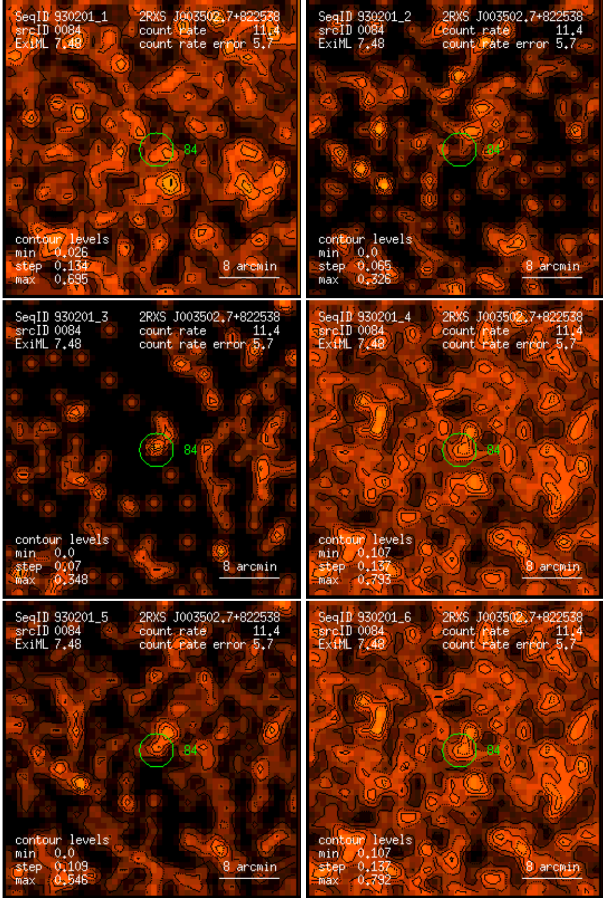
Figure 84: RASS 930201: detection 0084: band rate images, Gaussian filter: (1) PSPC channels 11 – 41, (2) 52 – 90, (3) 91 – 201, (4) 11 – 235, (5) 52 – 201, (6) 11 – 201. Broad band rates in counts/ks. Band rate contour levels in counts/ks/arcmin 2 .
