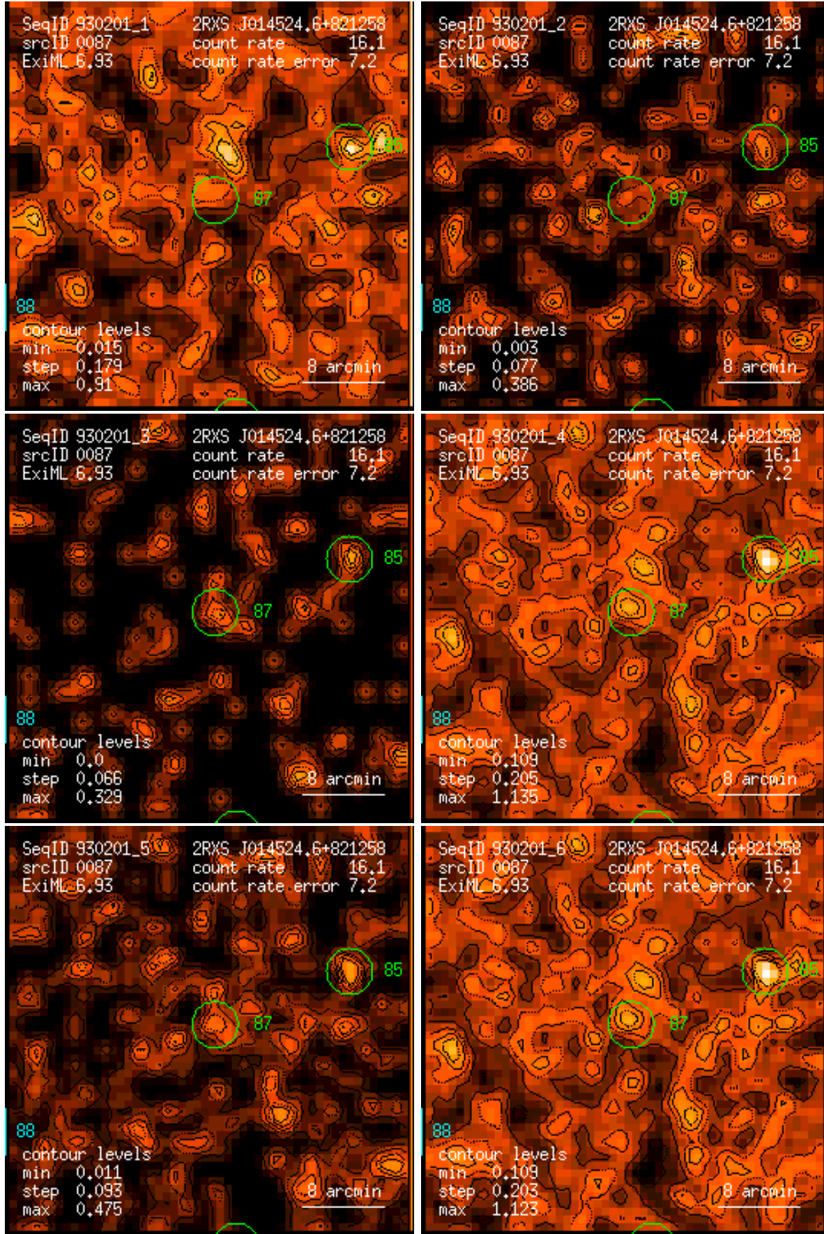
Figure 87: RASS 930201: detection 0087: band rate images, Gaussian filter: (1) PSPC channels 11 – 41, (2) 52 – 90, (3) 91 – 201, (4) 11 – 235, (5) 52 – 201, (6) 11 – 201. Broad band rates in counts/ks. Band rate contour levels in counts/ks/arcmin 2 .
