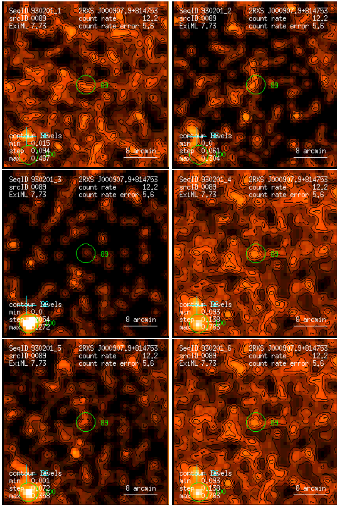
Figure 89: RASS 930201: detection 0089: band rate images, Gaussian filter: (1) PSPC channels 11 – 41, (2) 52 – 90, (3) 91 – 201, (4) 11 – 235, (5) 52 – 201, (6) 11 – 201. Broad band rates in counts/ks. Band rate contour levels in counts/ks/arcmin 2 .
