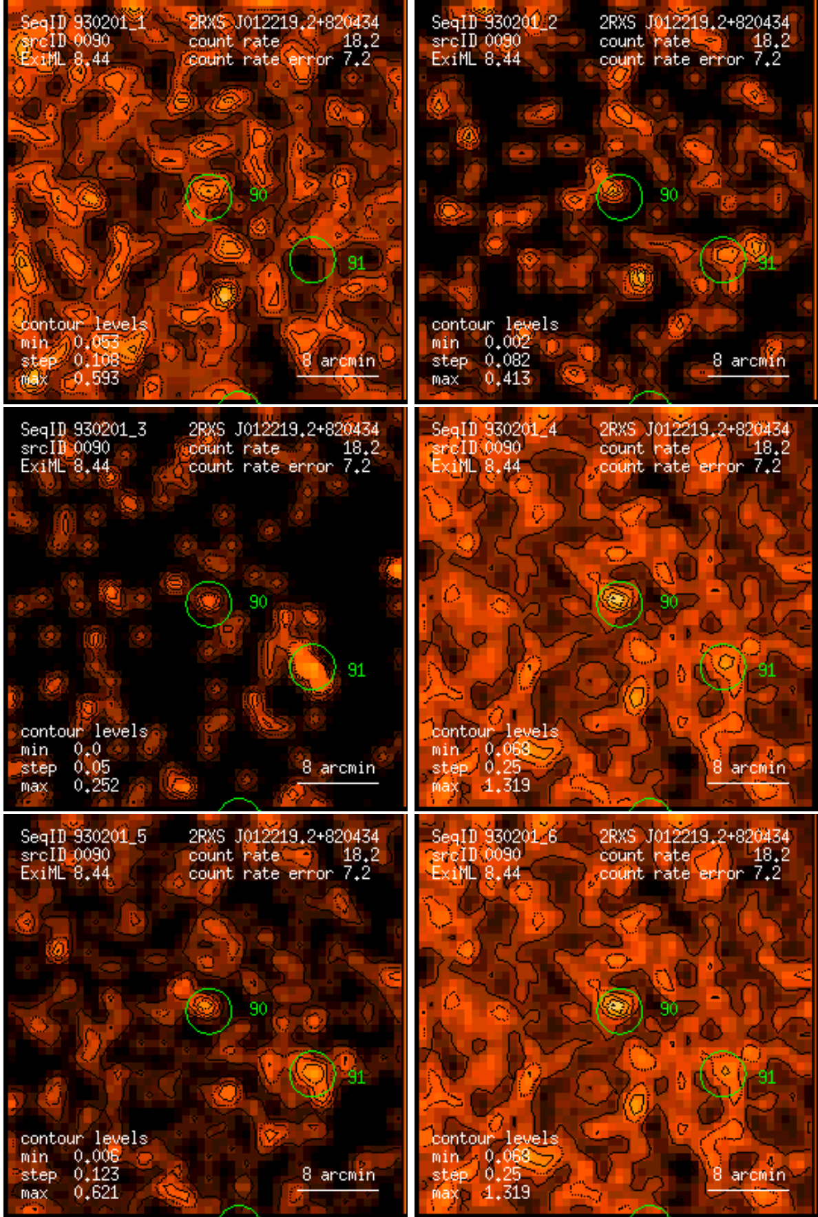
Figure 90: RASS 930201: detection 0090: band rate images, Gaussian filter: (1) PSPC channels 11 – 41, (2) 52 – 90, (3) 91 – 201, (4) 11 – 235, (5) 52 – 201, (6) 11 – 201. Broad band rates in counts/ks. Band rate contour levels in counts/ks/arcmin 2 .
