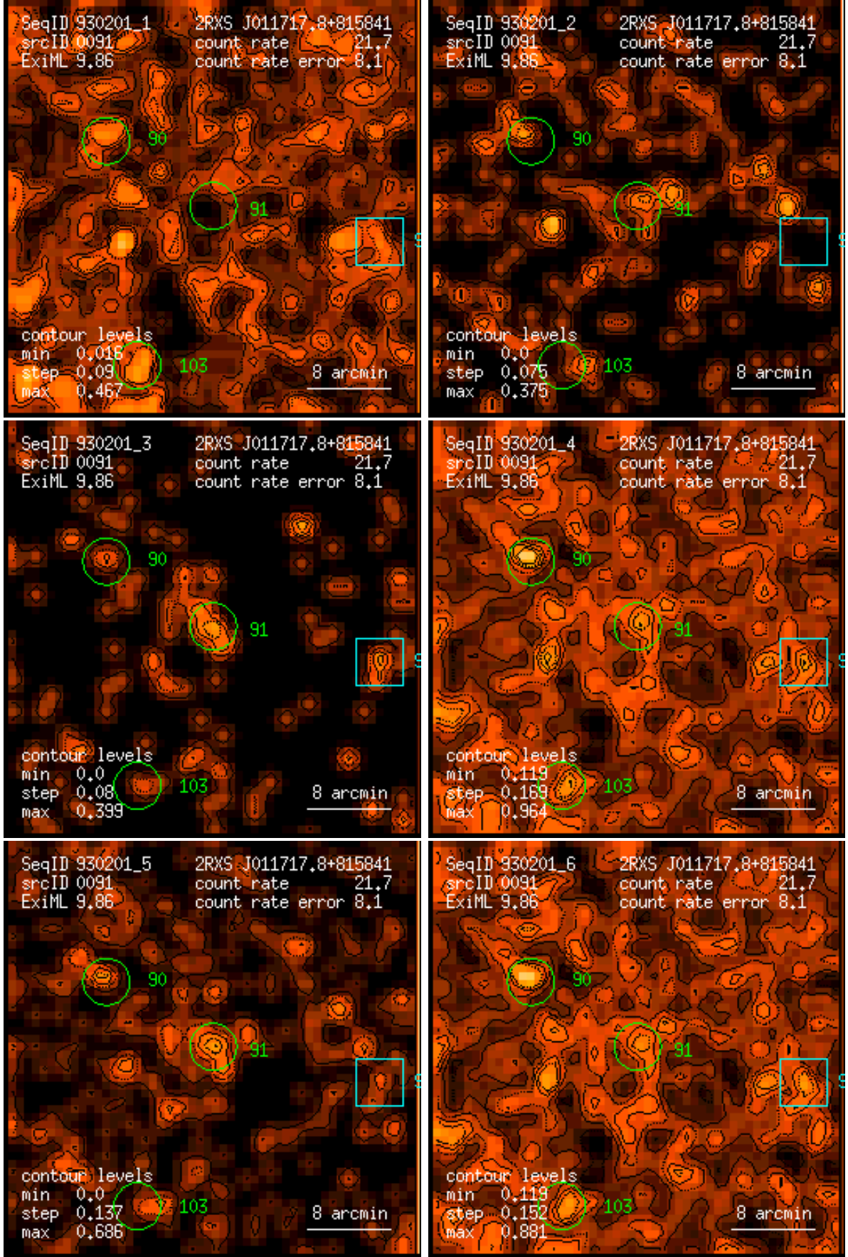
Figure 91: RASS 930201: detection 0091: band rate images, Gaussian filter: (1) PSPC channels 11 – 41, (2) 52 – 90, (3) 91 – 201, (4) 11 – 235, (5) 52 – 201, (6) 11 – 201. Broad band rates in counts/ks. Band rate contour levels in counts/ks/arcmin 2 .
