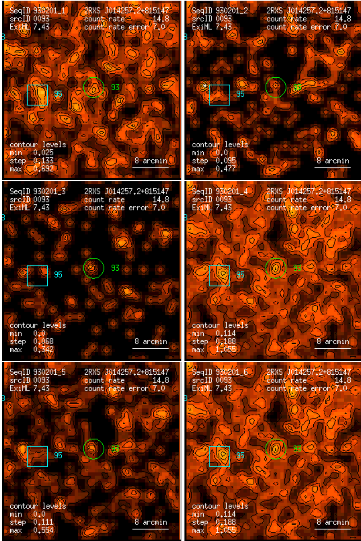
Figure 93: RASS 930201: detection 0093: band rate images, Gaussian filter: (1) PSPC channels 11 – 41, (2) 52 – 90, (3) 91 – 201, (4) 11 – 235, (5) 52 – 201, (6) 11 – 201. Broad band rates in counts/ks. Band rate contour levels in counts/ks/arcmin 2 .
