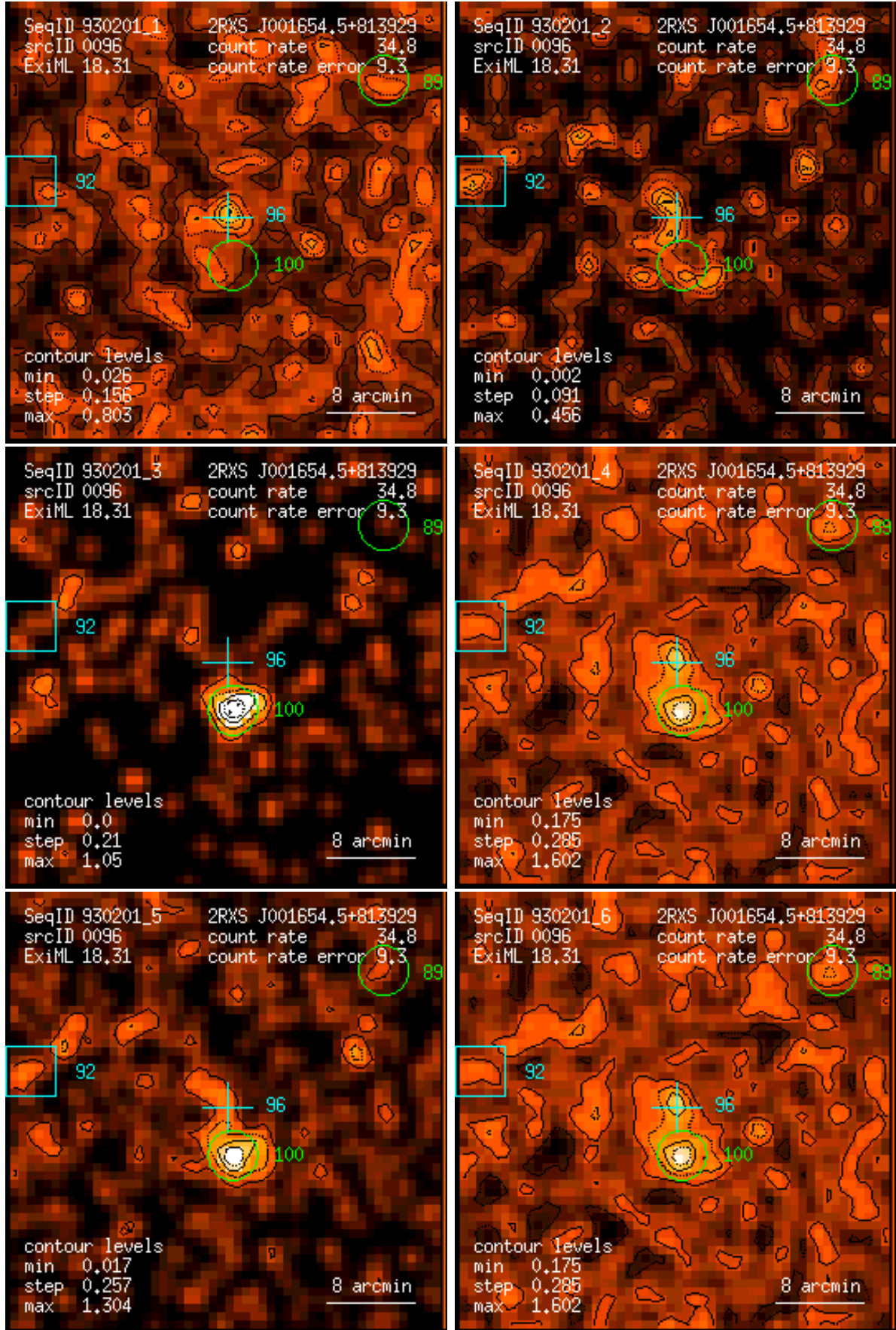
Figure 96: RASS 930201: detection 0096: band rate images, Gaussian filter: (1) PSPC channels 11 – 41, (2) 52 – 90, (3) 91 – 201, (4) 11 – 235, (5) 52 – 201, (6) 11 – 201. Broad band rates in counts/ks. Band rate contour levels in counts/ks/arcmin 2 .
