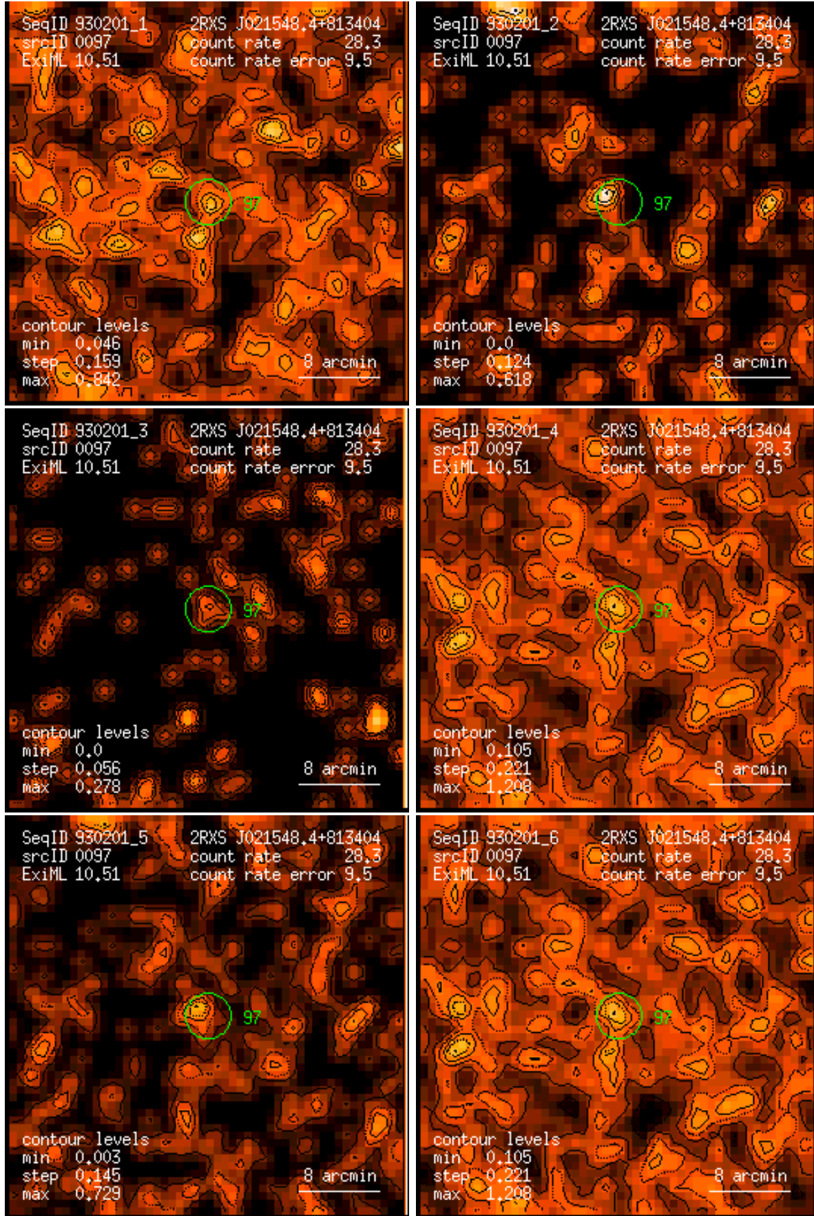
Figure 97: RASS 930201: detection 0097: band rate images, Gaussian filter: (1) PSPC channels 11 – 41, (2) 52 – 90, (3) 91 – 201, (4) 11 – 235, (5) 52 – 201, (6) 11 – 201. Broad band rates in counts/ks. Band rate contour levels in counts/ks/arcmin 2 .
