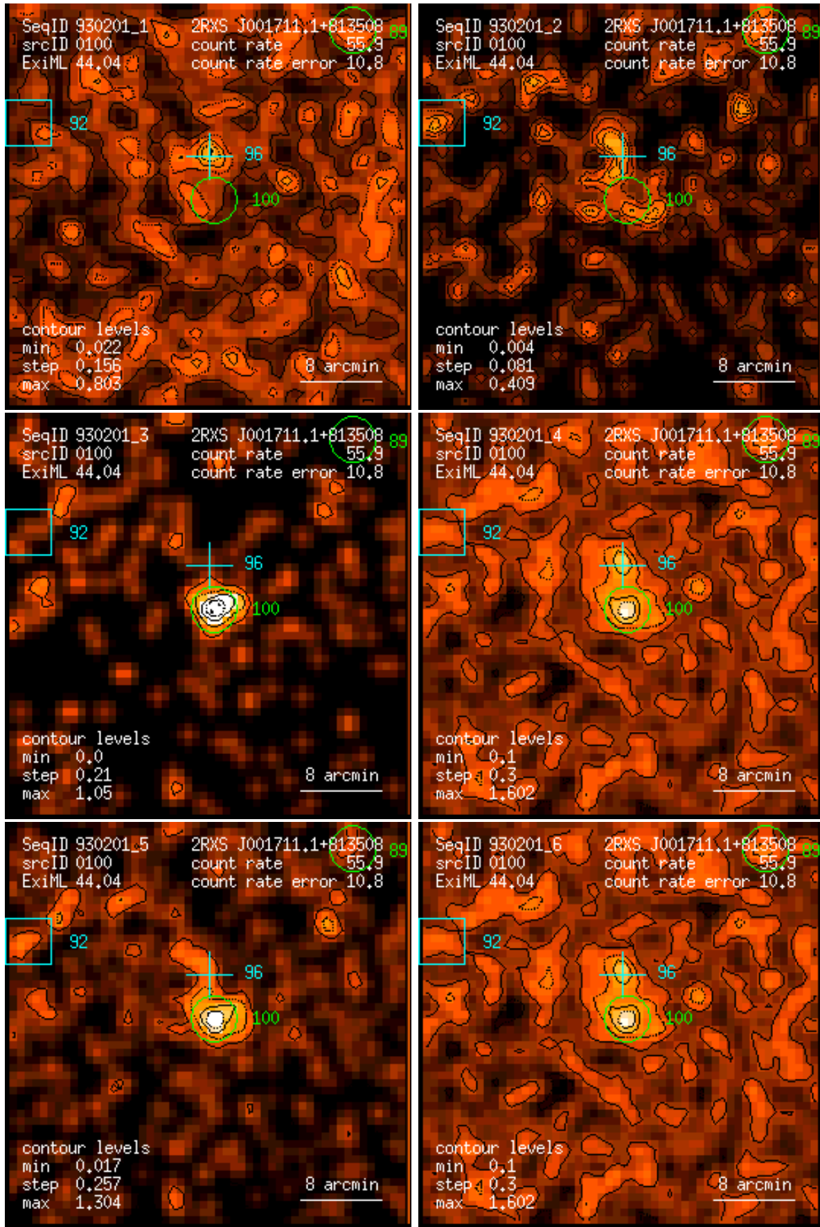
Figure 100: RASS 930201: detection 0100: band rate images, Gaussian filter: (1) PSPC channels 11 – 41, (2) 52 – 90, (3) 91 – 201, (4) 11 – 235, (5) 52 – 201, (6) 11 – 201. Broad band rates in counts/ks. Band rate contour levels in counts/ks/arcmin 2 .
