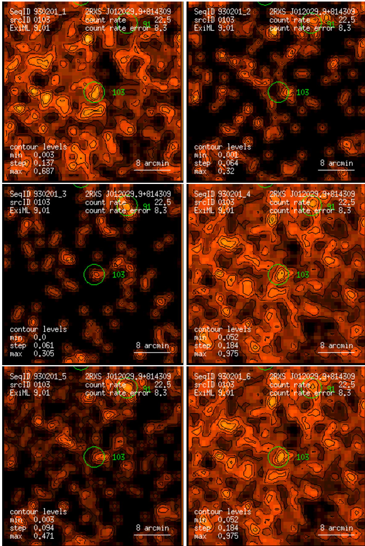
Figure 103: RASS 930201: detection 0103: band rate images, Gaussian filter: (1) PSPC channels 11 – 41, (2) 52 – 90, (3) 91 – 201, (4) 11 – 235, (5) 52 – 201, (6) 11 – 201. Broad band rates in counts/ks. Band rate contour levels in counts/ks/arcmin 2 .
