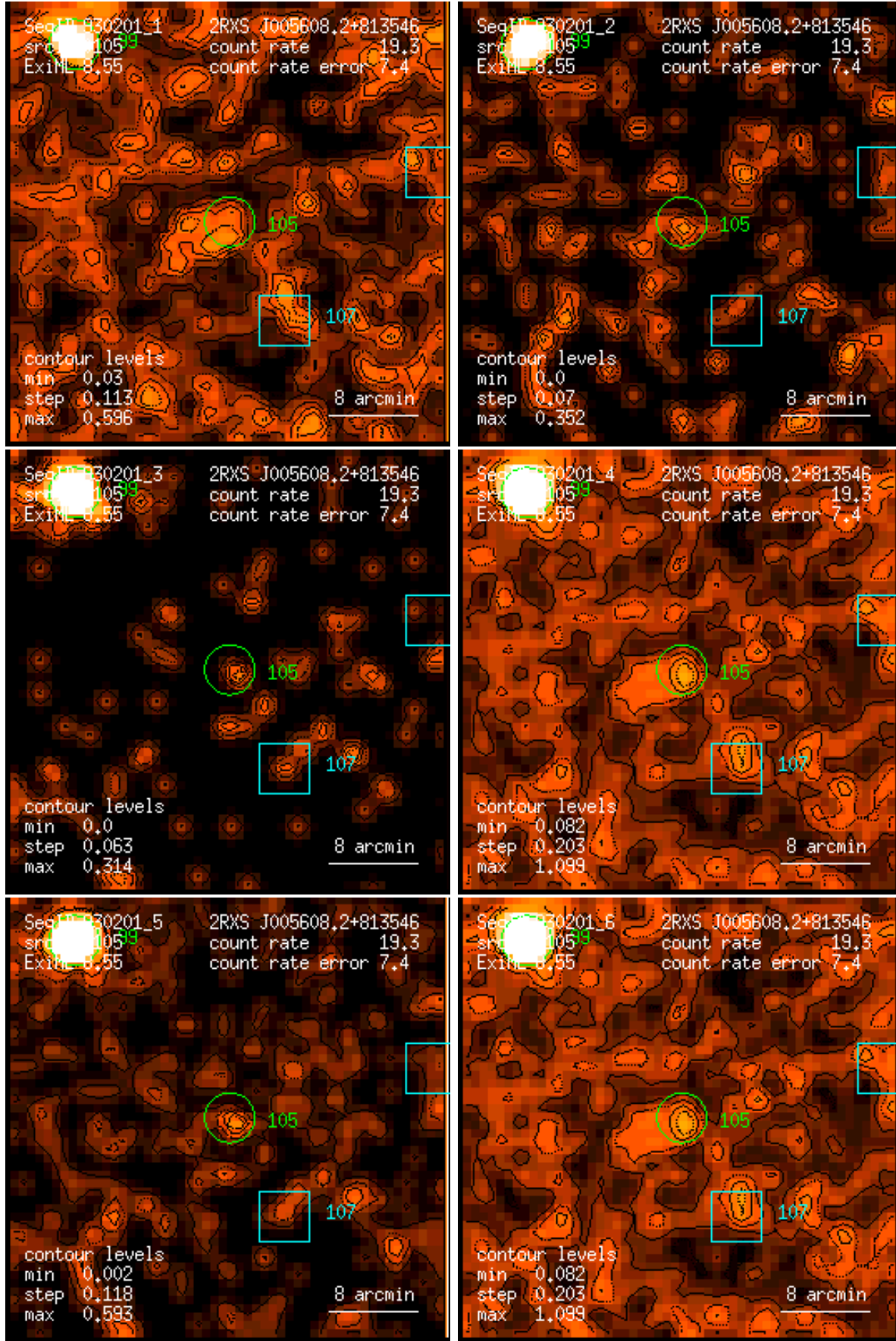
Figure 105: RASS 930201: detection 0105: band rate images, Gaussian filter: (1) PSPC channels 11 – 41, (2) 52 – 90, (3) 91 – 201, (4) 11 – 235, (5) 52 – 201, (6) 11 – 201. Broad band rates in counts/ks. Band rate contour levels in counts/ks/arcmin 2 .
