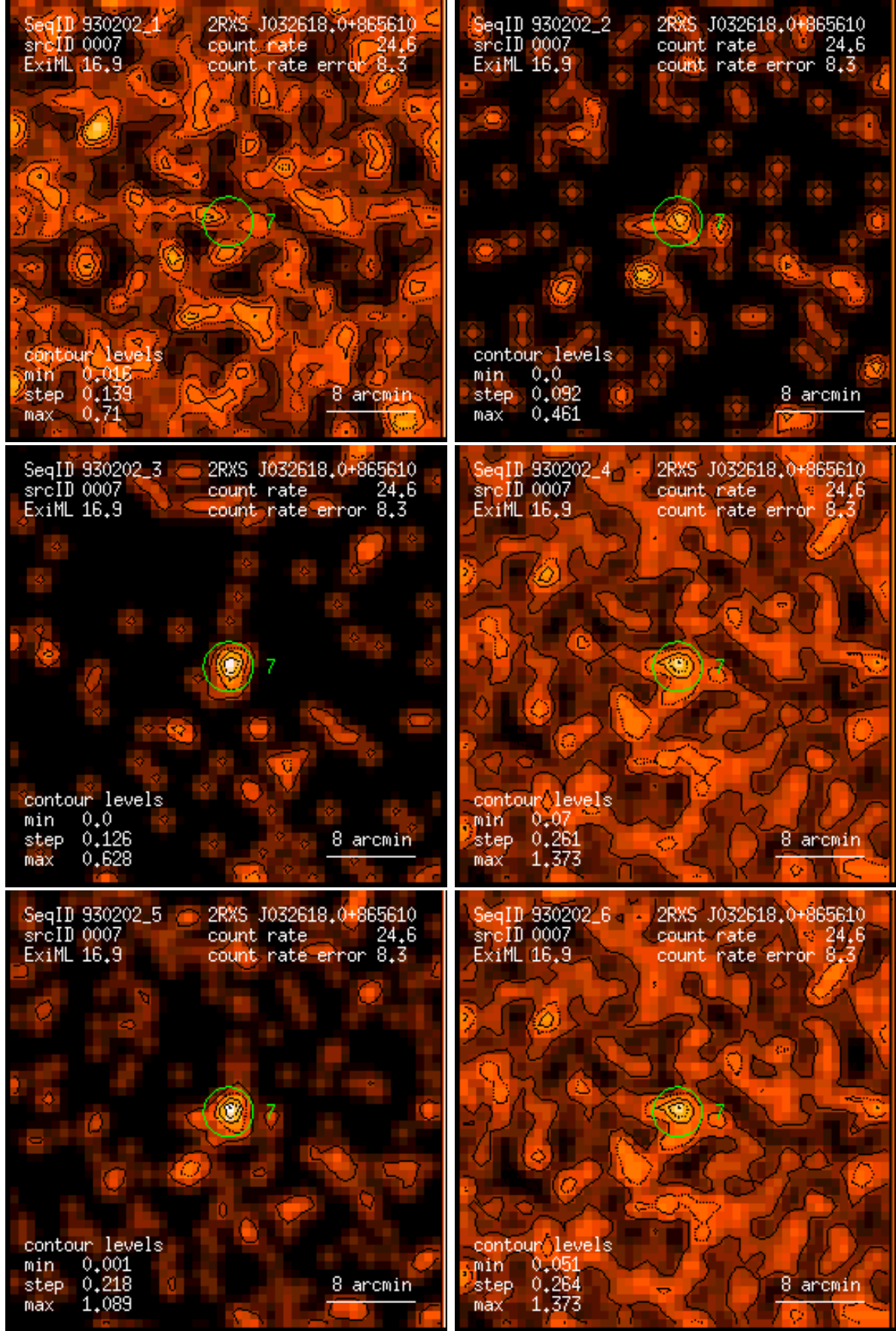
Figure 7: RASS 930202: detection 0007: band rate images, Gaussian filter: (1) PSPC channels 11 – 41, (2) 52 – 90, (3) 91 – 201, (4) 11 – 235, (5) 52 – 201, (6) 11 – 201. Broad band rates in counts/ks. Band rate contour levels in counts/ks/arcmin 2 .
