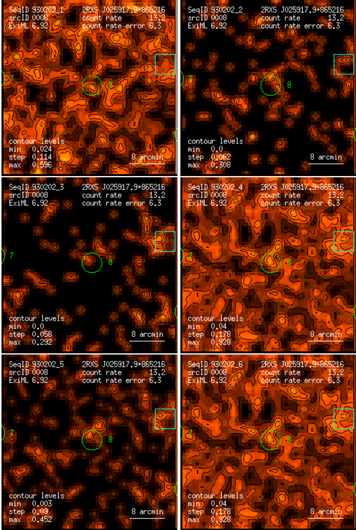
Figure 8: RASS 930202: detection 0008: band rate images, Gaussian filter: (1) PSPC channels 11 – 41, (2) 52 – 90, (3) 91 – 201, (4) 11 – 235, (5) 52 – 201, (6) 11 – 201. Broad band rates in counts/ks. Band rate contour levels in counts/ks/arcmin 2 .
